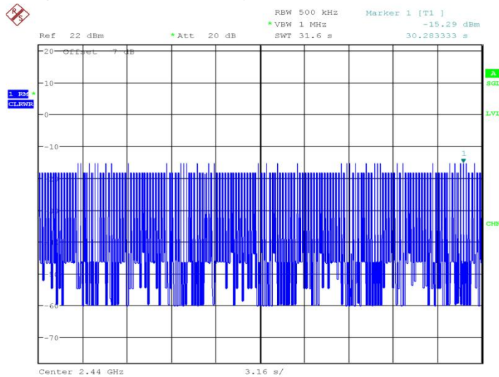
Fig.57 Time of occupancy (Dwell Time): Ch39,Packet 3-DH1
