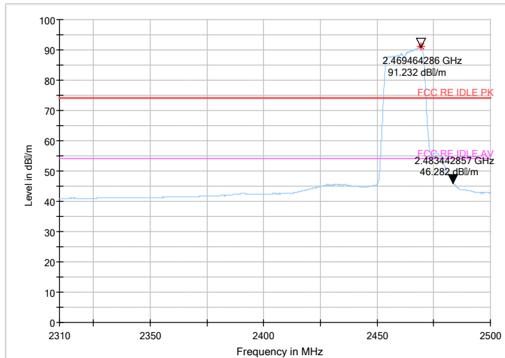
Fig.49 Radiated emission (Power): 802.11g, high channel
