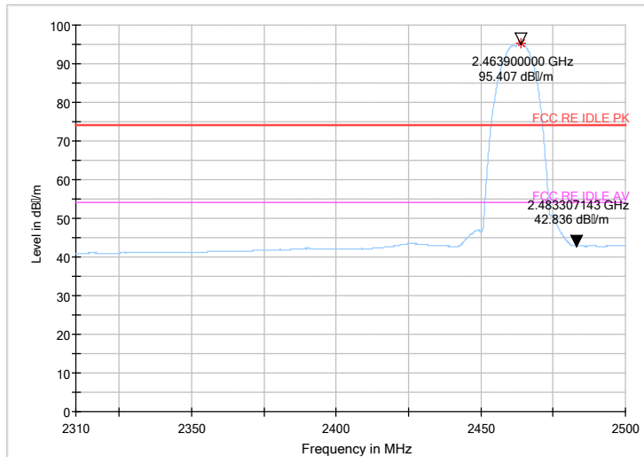
Fig.44 Radiated emission (Power): 802.11b, high channel
