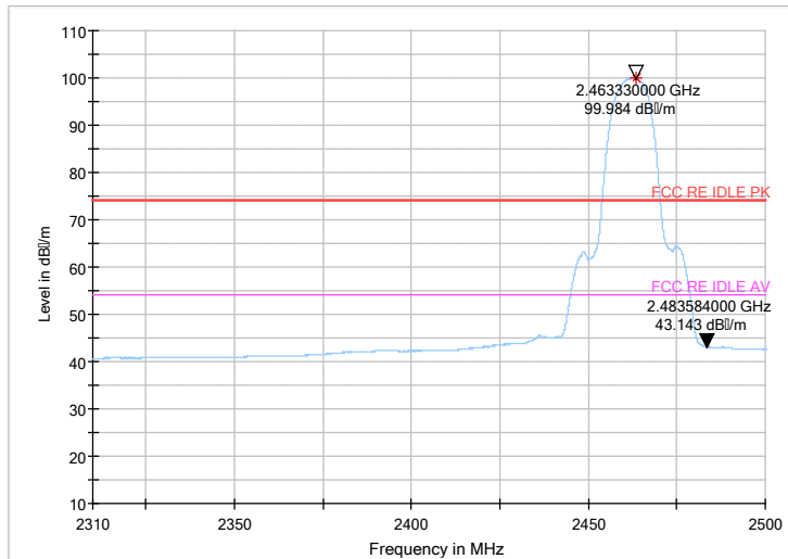
Fig.59 Radiated emission (Power): 802.11b, high channel
