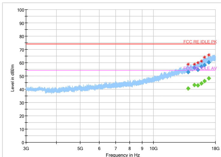
Fig.23 Radiated emission: Ch39, 3GHz~18GHz
