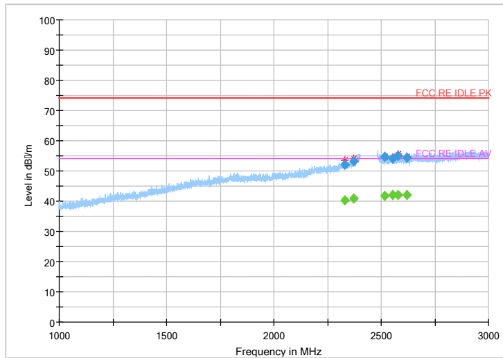
Fig.25 Radiated emission: Ch39, 1GHz~3GHz
