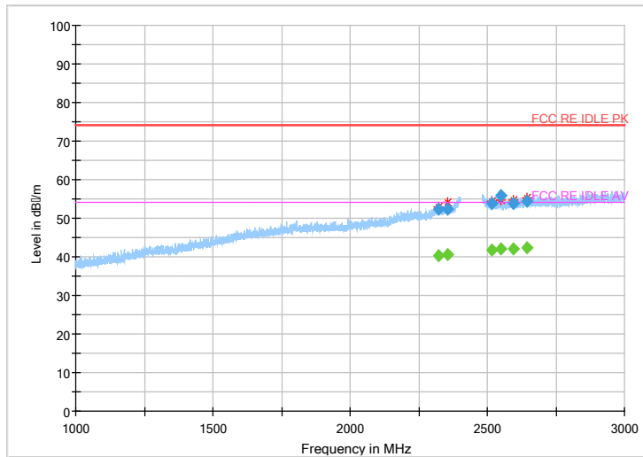
Fig.22 Radiated emission: Ch39, 1GHz~3GHz
