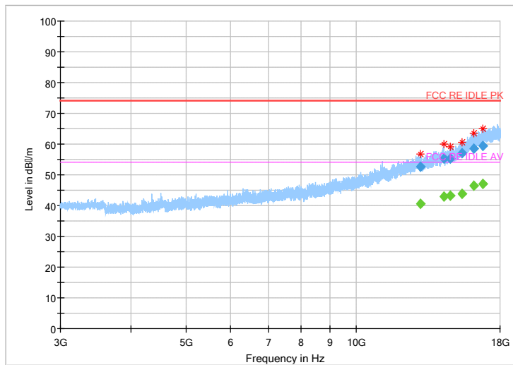
Fig.26 Radiated emission: Ch39, 3GHz~18GHz
