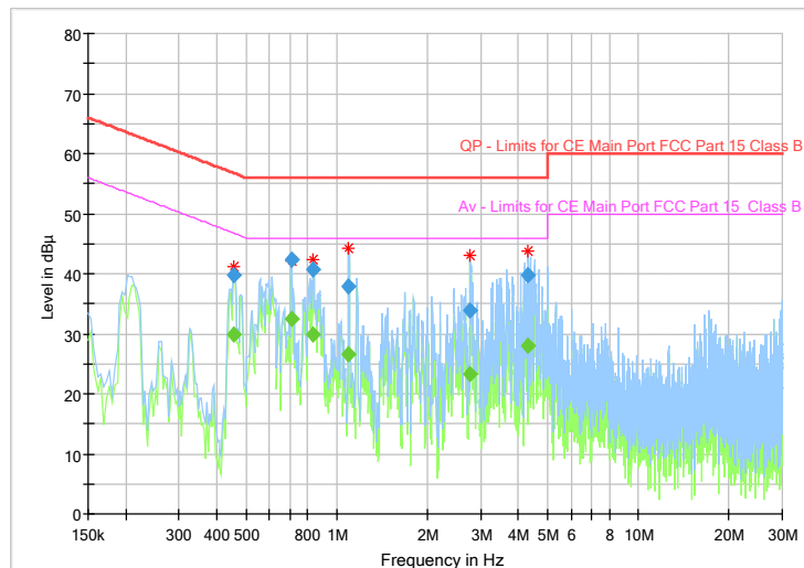
Fig.24 AC Powerline Conducted Emission
