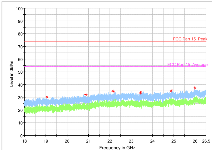
Fig. 51 Radiated Spurious Emission (802.11 n-HT20, ch64, 18 GHz-26.5 GHz)
