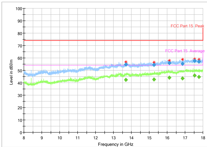
Fig. 36 Radiated Spurious Emission (802.11a, ch52, 8 GHz-18 GHz)
