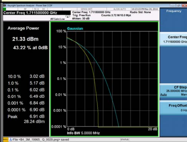
3MHz / 16QAM
