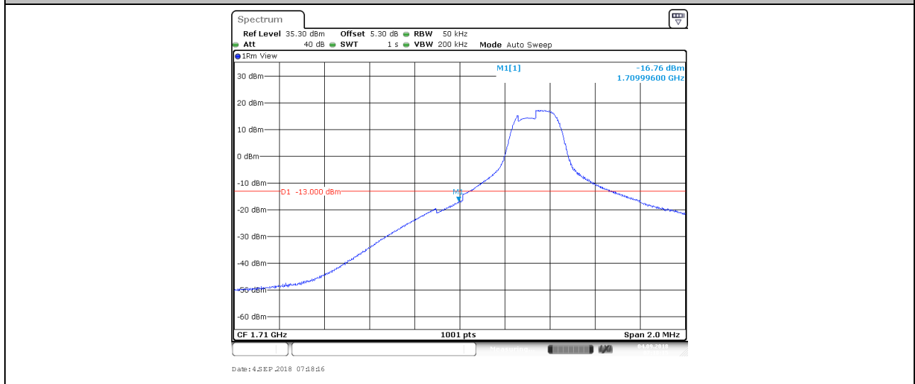
BAND4_5MHz_16QAM_19975_1RB#24
