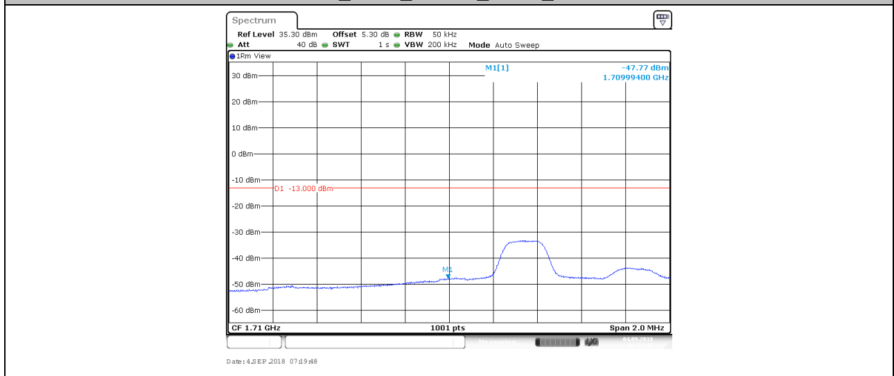
BAND4_5MHz_16QAM_19975_25RB#0
