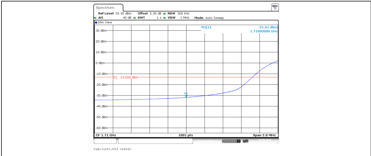
BAND4_20MHz_QPSK_20300_1RB#0
