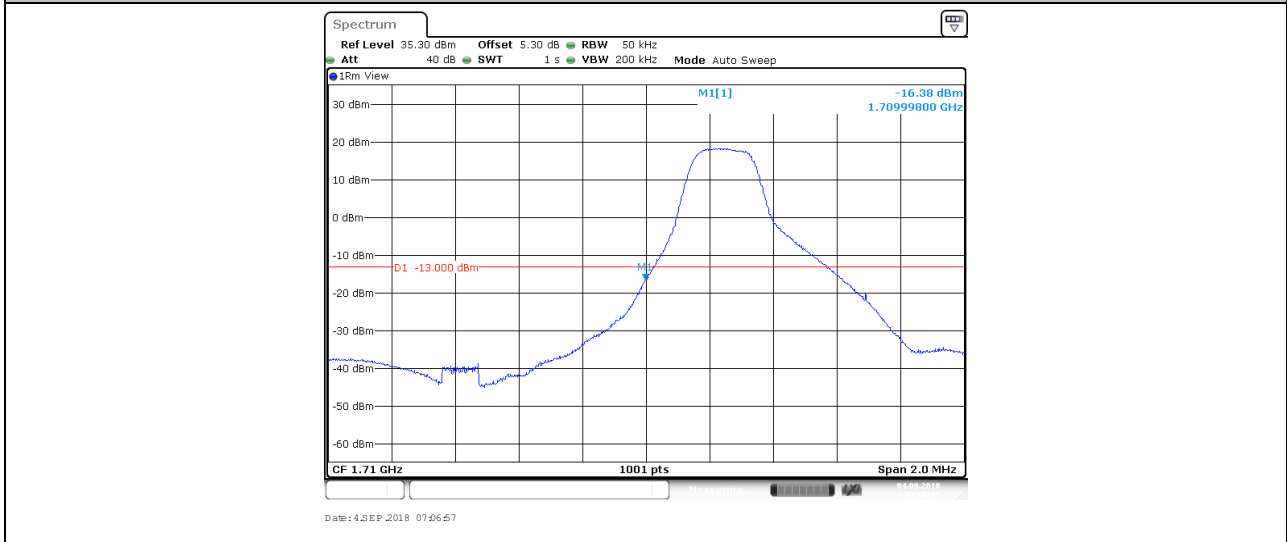
BAND4_3MHz_16QAM_19965_1RB#14
