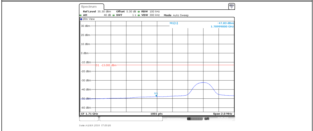
BAND4_10MHz_16QAM_20000_50RB#0
