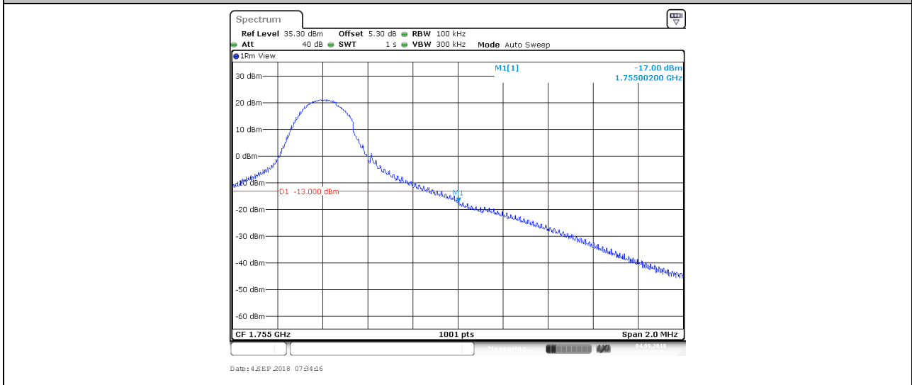
BAND4_10MHz_QPSK_20350_50RB#0
