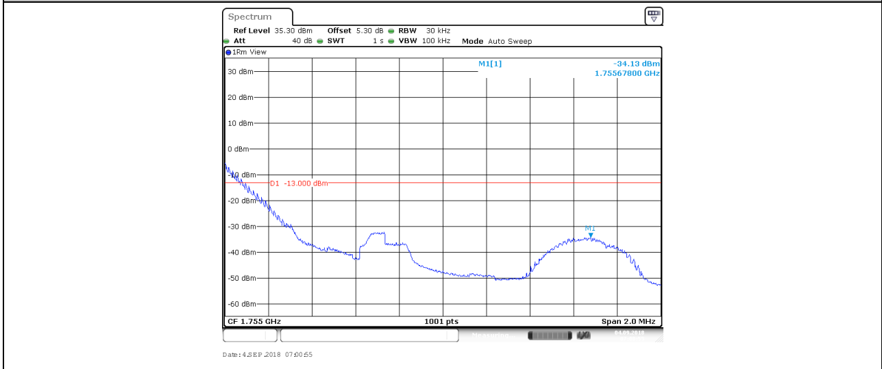
BAND4_1.4MHz_16QAM_20393_1RB#5
