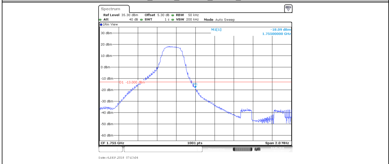
BAND4_3MHz_16QAM_20385_15RB#0
