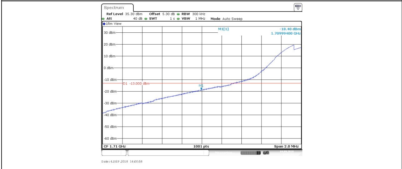
BAND4_20MHz_QPSK_20050_1RB#99
