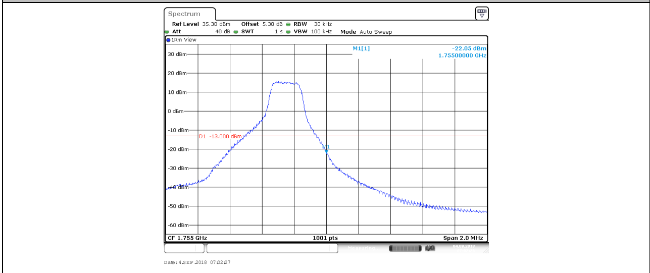
BAND4_1.4MHz_16QAM_20393_6RB#0
