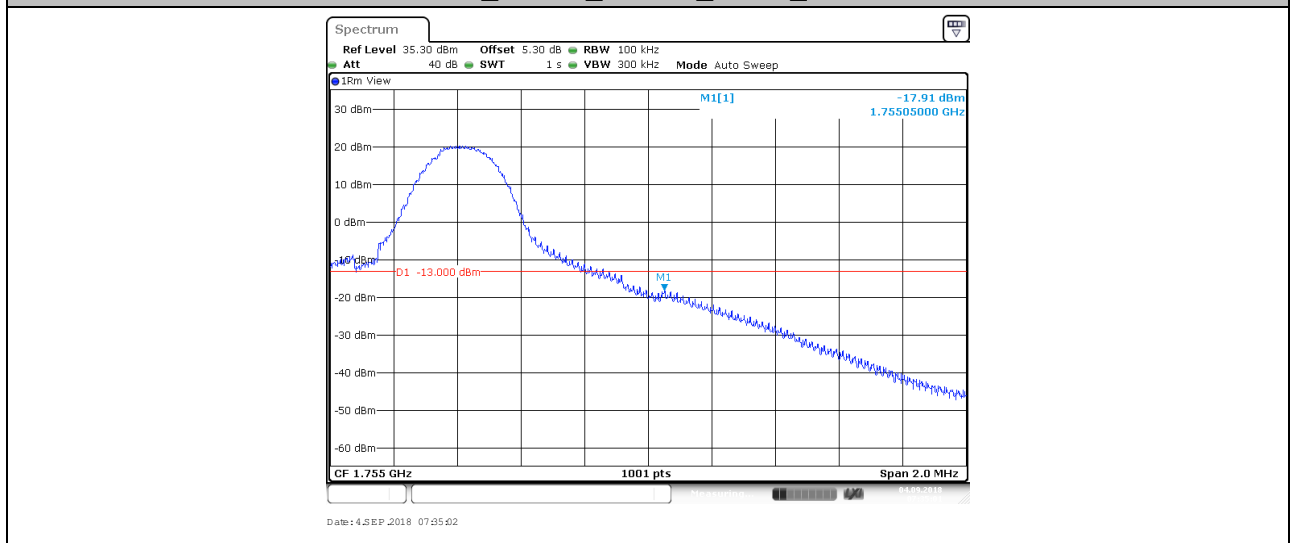
BAND4_10MHz_16QAM_20350_50RB#0
