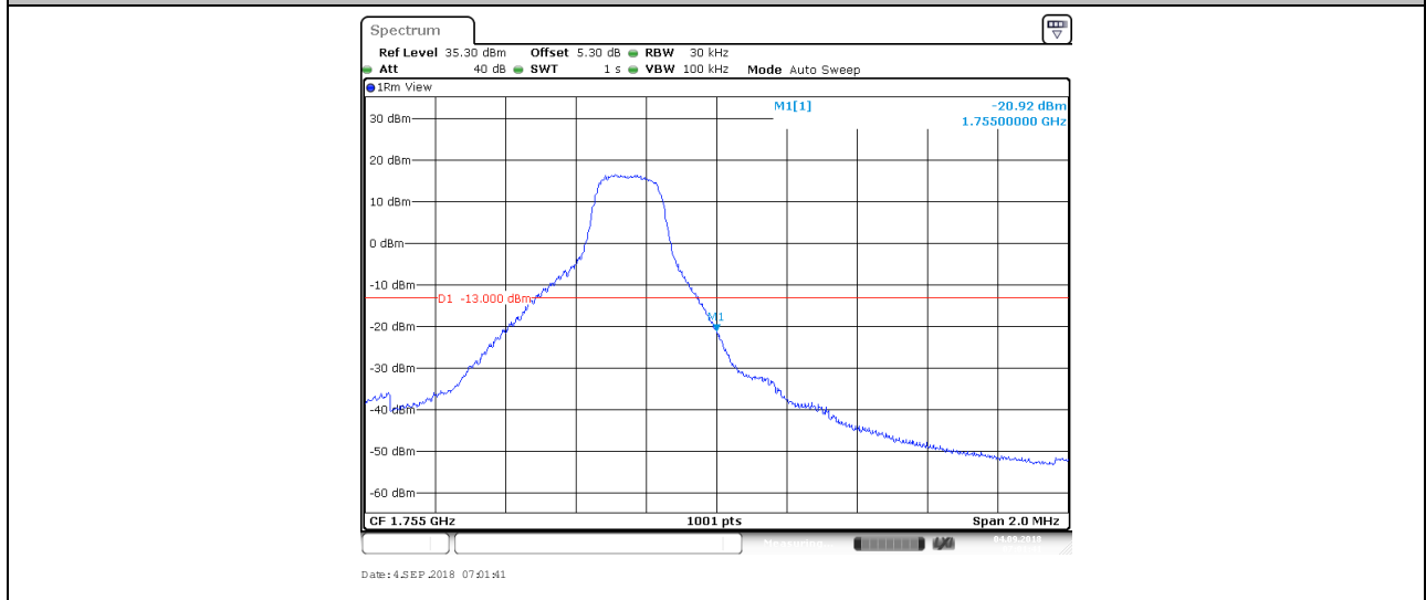
BAND4_1.4MHz_QPSK_20393_6RB#0
