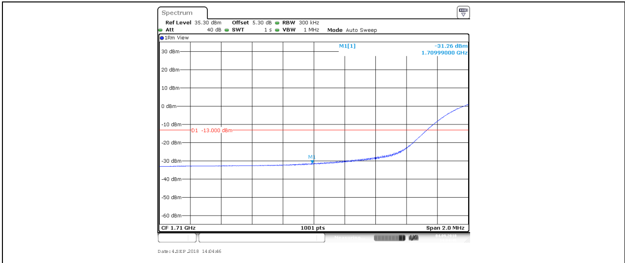
BAND4_20MHz_16QAM_20300_1RB#0
