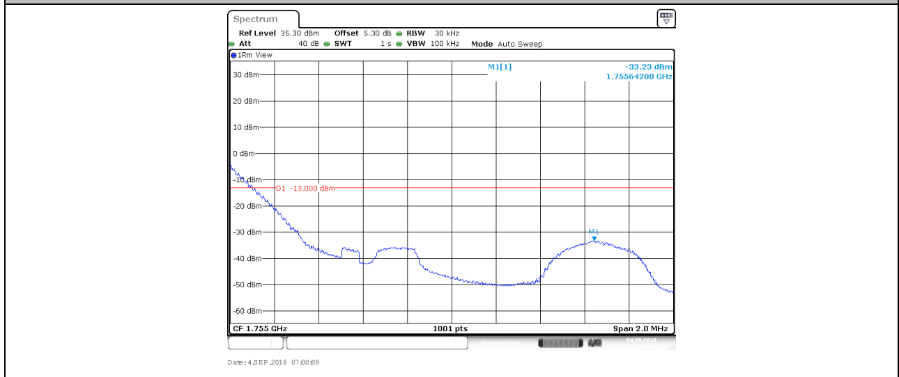
BAND4_1.4MHz_QPSK_20393_1RB#5
