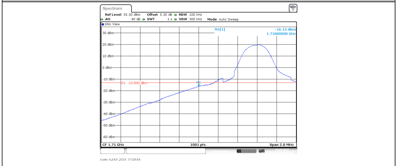
BAND4_10MHz_16QAM_20000_1RB#49
