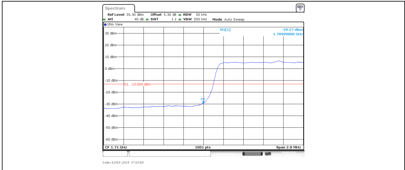
BAND4_3MHz_16QAM_20385_1RB#0
