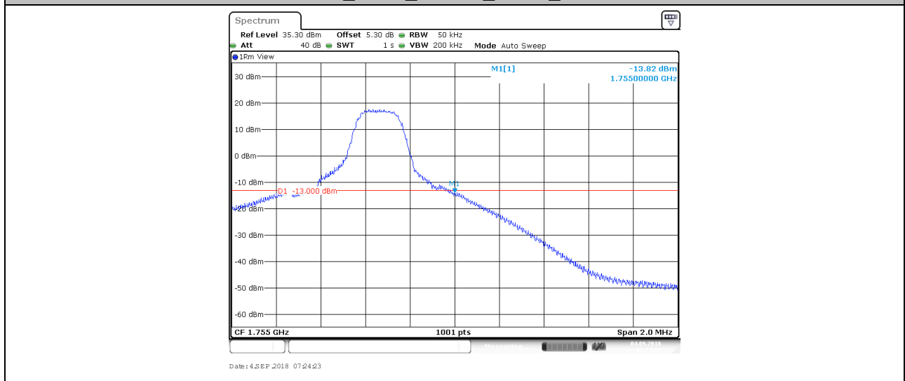
BAND4_5MHz_16QAM_20375_25RB#0
