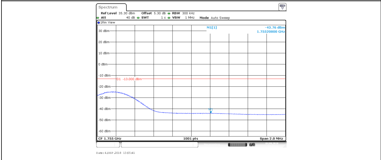
BAND4_15MHz_16QAM_20325_1RB#74
