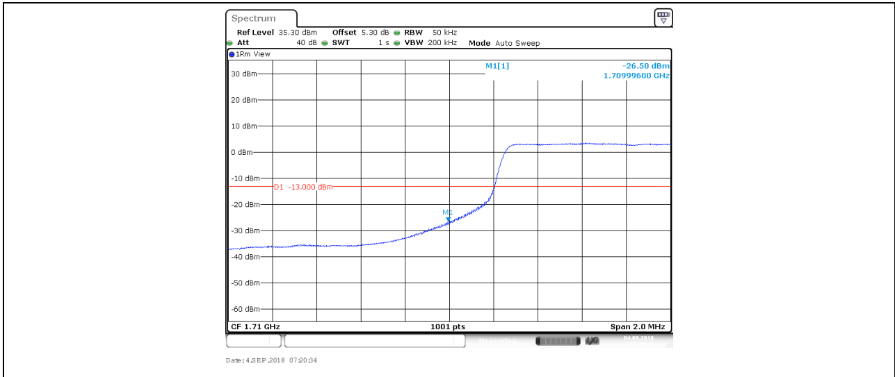
BAND4_5MHz_QPSK_20375_1RB#0
