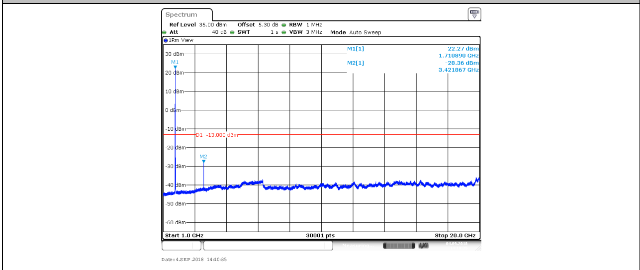
BAND4_20MHz_16QAM_20175_1RB#0
