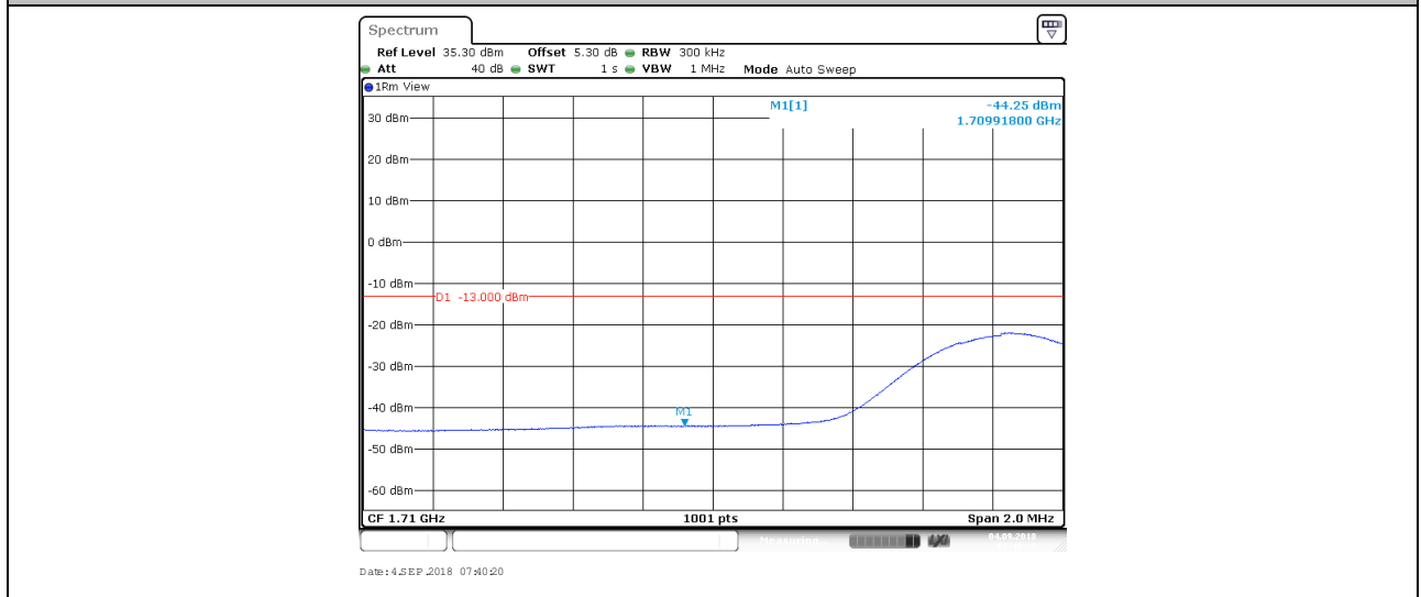
BAND4_15MHz_QPSK_20025_75RB#0
