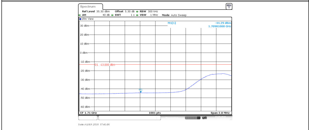
BAND4_15MHz_16QAM_20025_75RB#0
