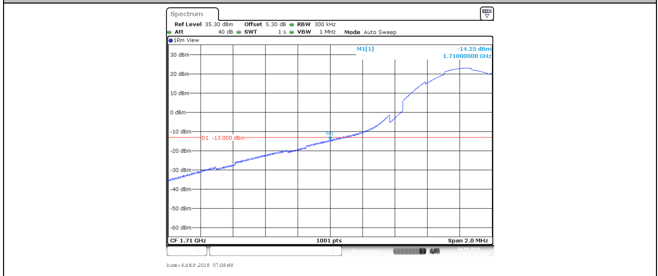
BAND4_15MHz_QPSK_20025_1RB#74
