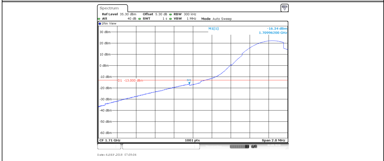
BAND4_15MHz_16QAM_20025_1RB#74
