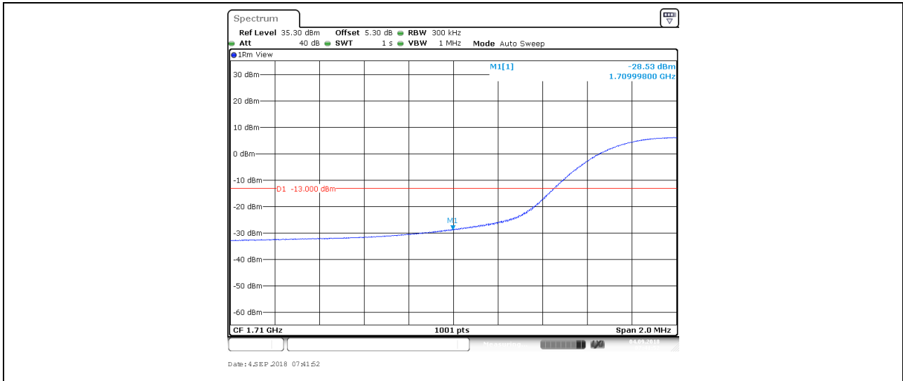
BAND4_15MHz_QPSK_20325_1RB#0
