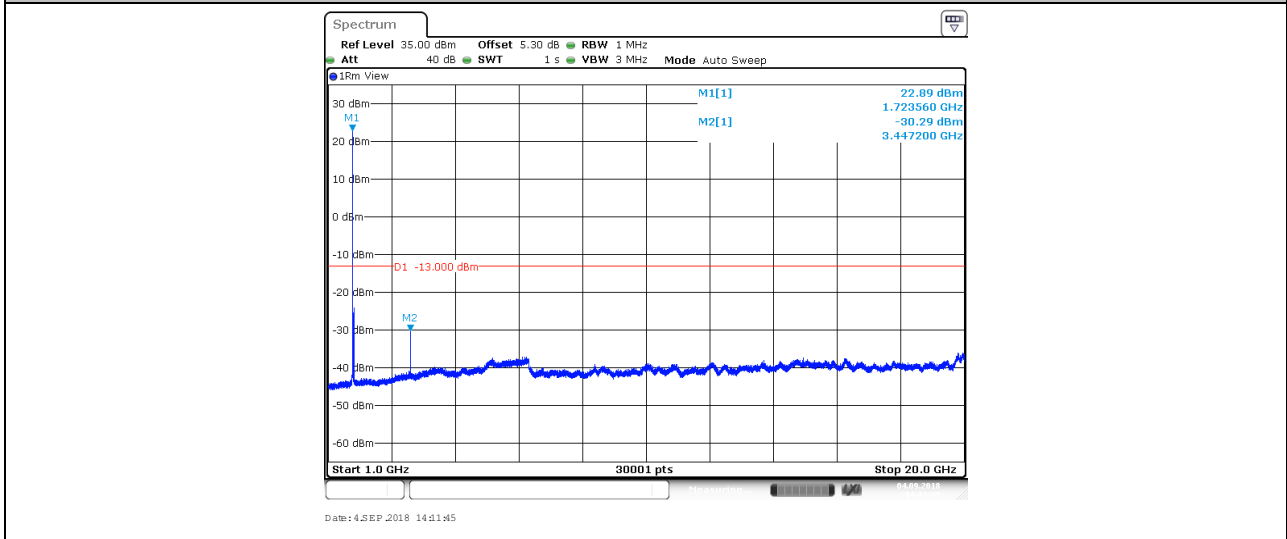
BAND4_20MHz_16QAM_20300_1RB#0
