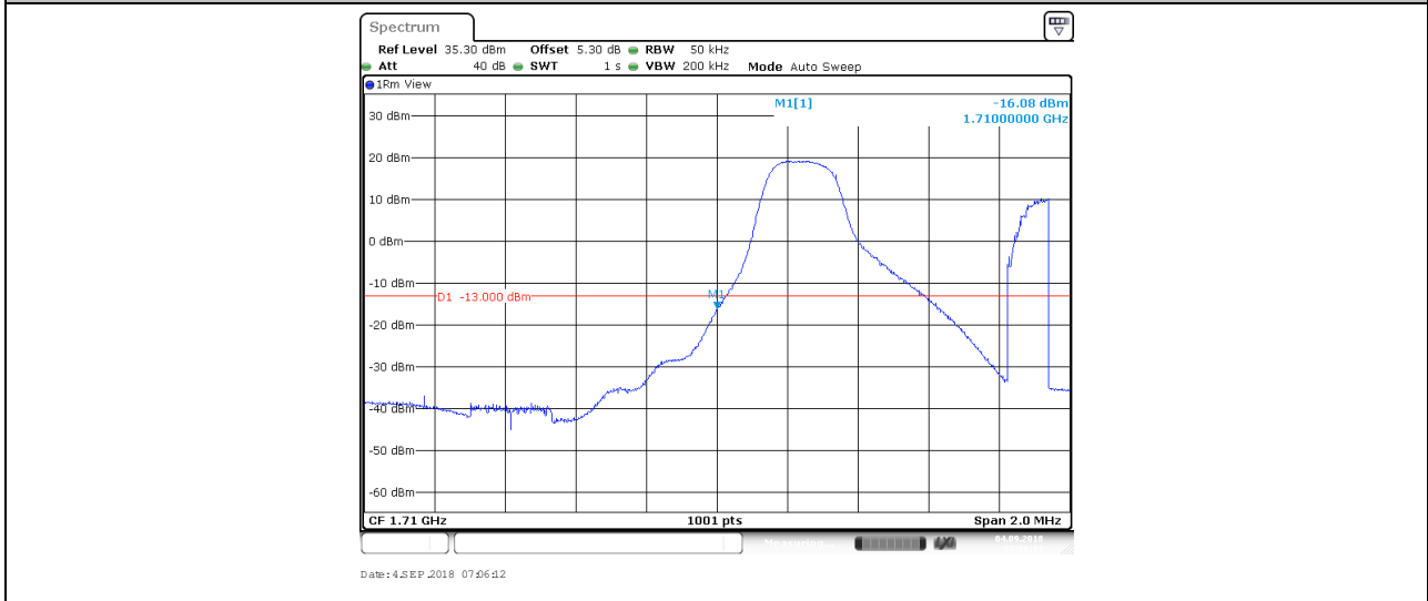
BAND4_3MHz_QPSK_19965_1RB#14
