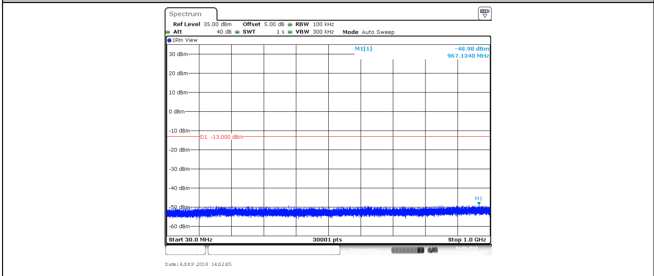
BAND4_20MHz_QPSK_20300_1RB#
