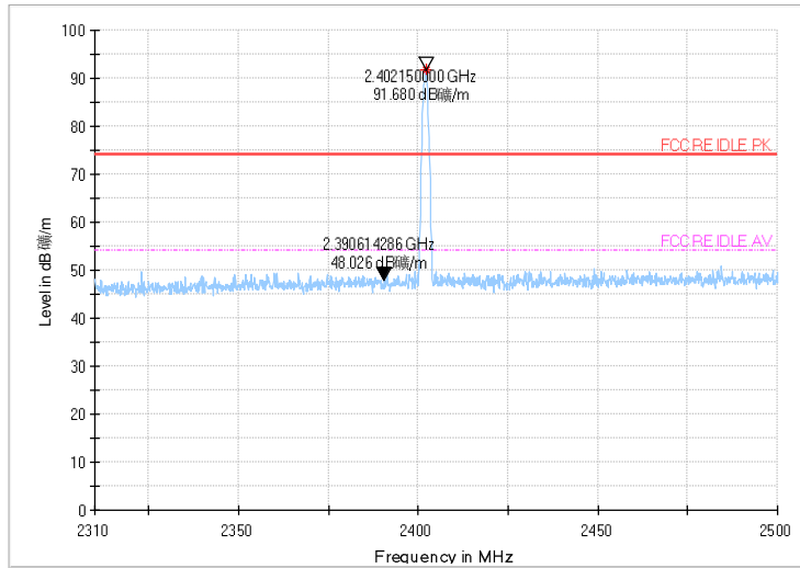
BANDEDGE: GFSK, Ch0,PK
