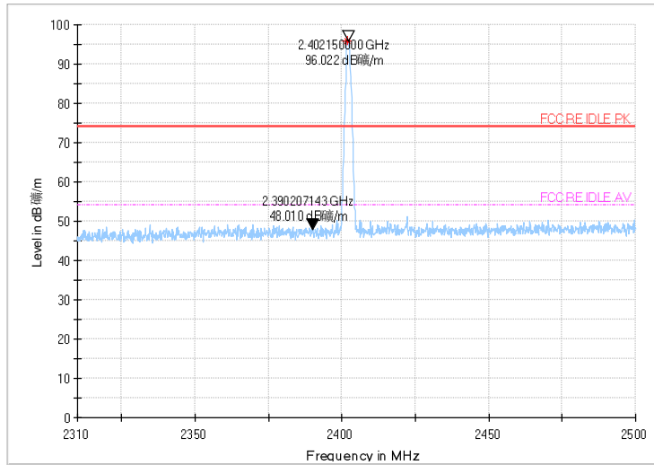
BANEDGE: 8DPSK, Ch0,PK
