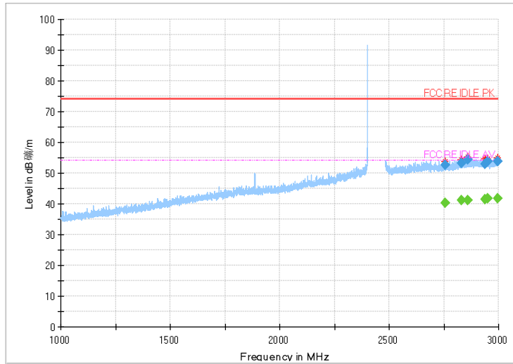
Fig.44 Radiated emission: \pi/4 DQPSK, Ch0, 1GHz~3GHz
