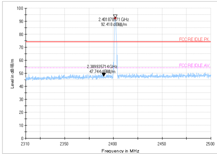
BANDEDGE: \pi/4 DQPSK, Ch0,PK
