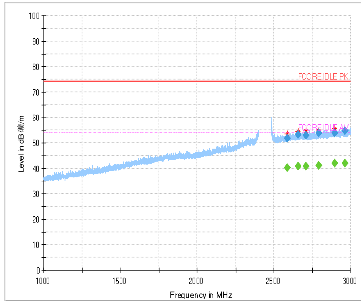
Fig.56 Radiated Spurious Emission (802.11 n-20MHz,Ch11,1GHz~3GHz)
