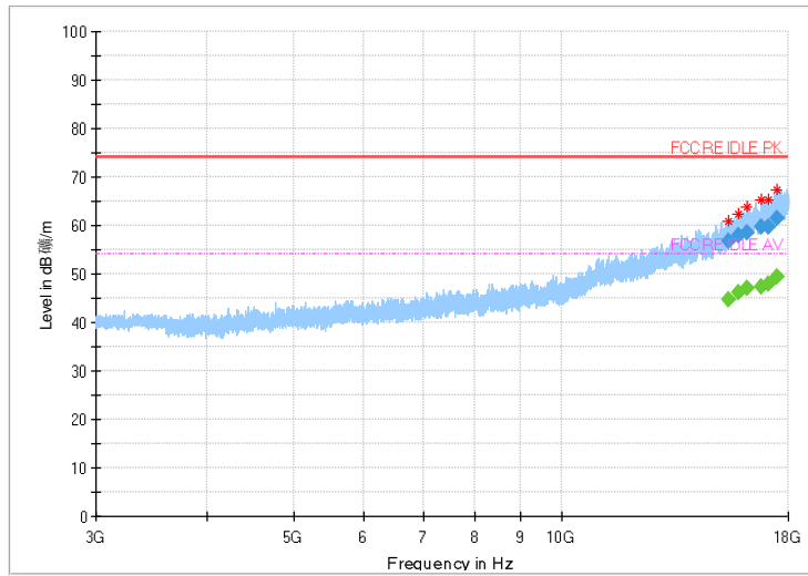
Fig.53 Radiated Spurious Emission (802.11g,Ch13,3GHz~18GHz)
