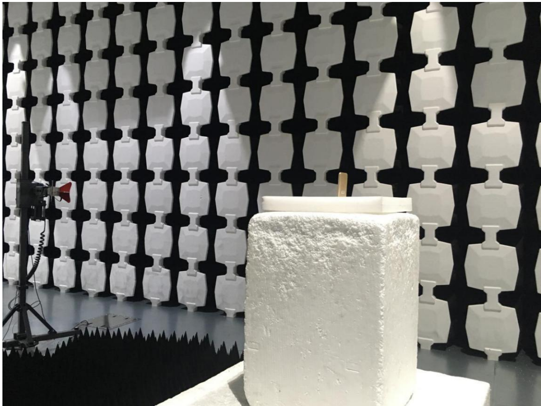
Description: Radiated Emission Test Setup (1-18GHz)
