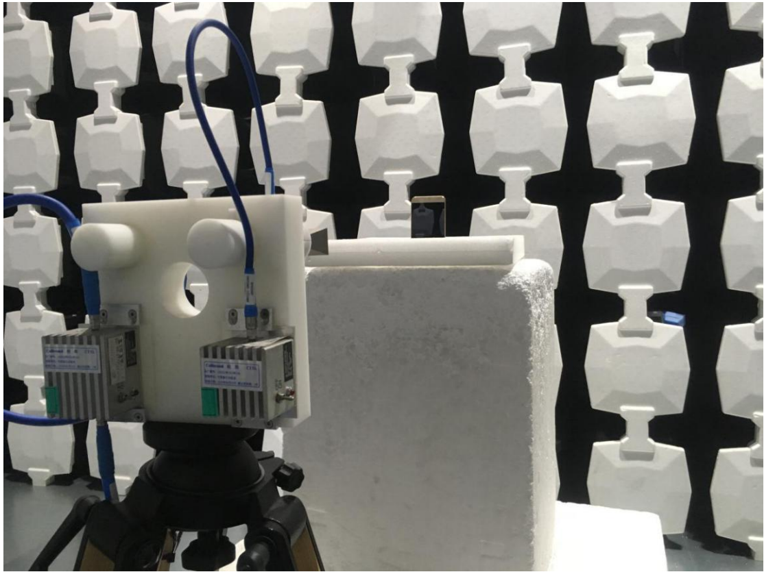
Description: Radiated Emission Test Setup (Above 18GHz)
