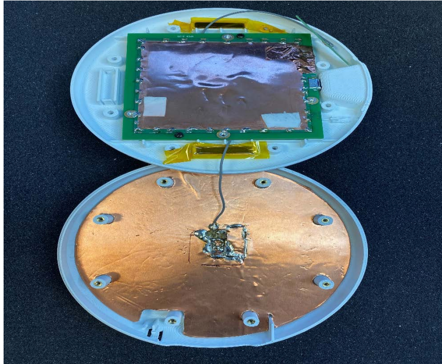
WPT Antenna Top View
