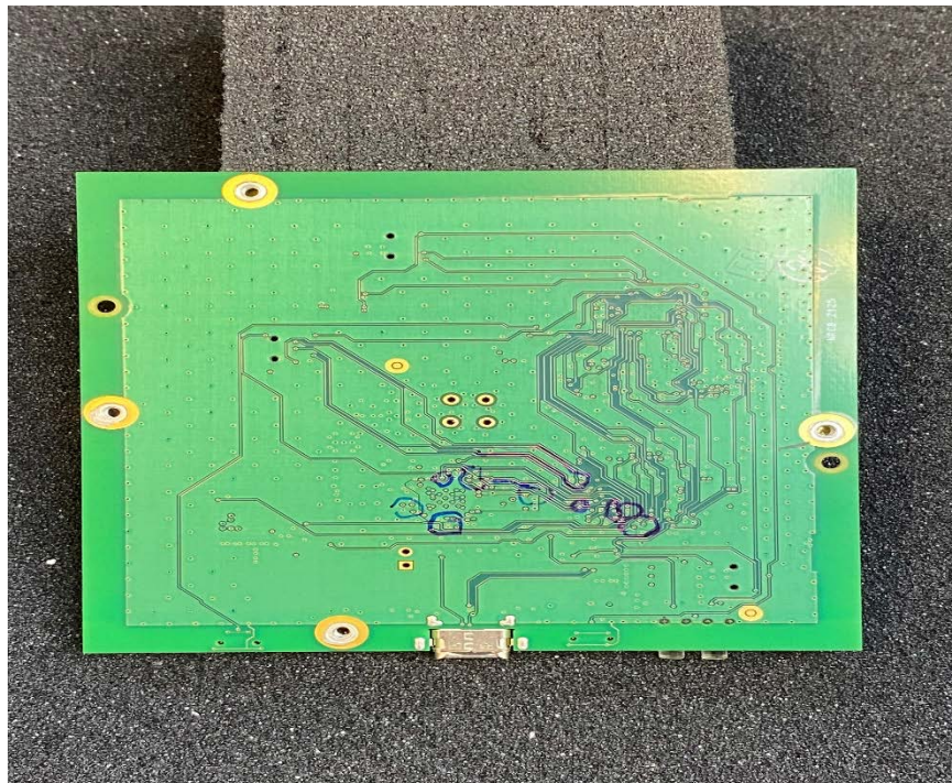
PCB Bottom View with No Shield
