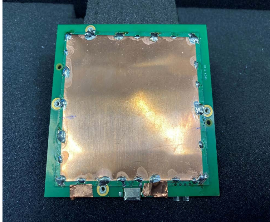
PCB Bottom View with Shield
