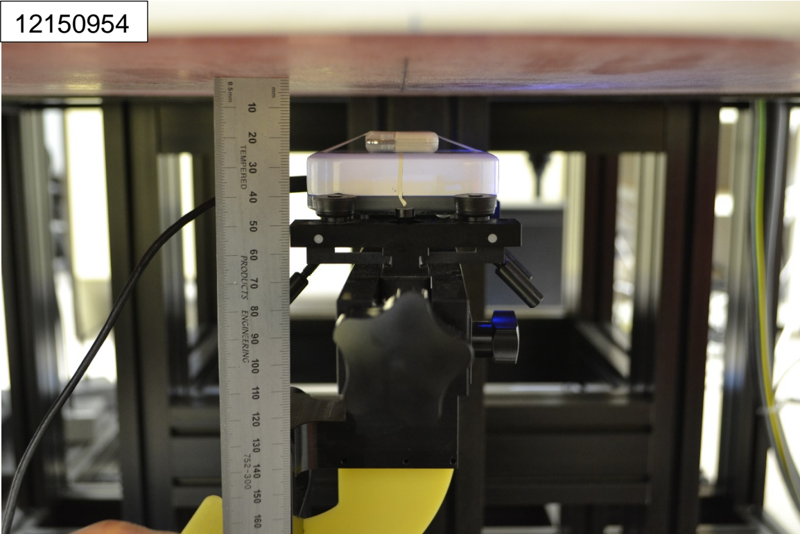
Antenna 2: Top @25mm
