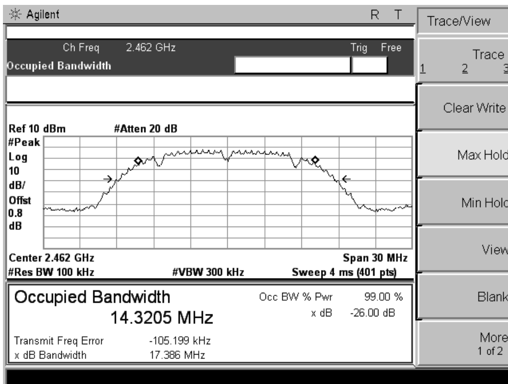
802.11g channel, 99% Occupied Bandwidth / Port.1+Port.2
