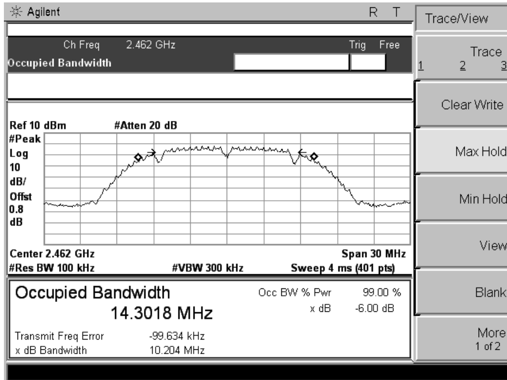
802.11g channel, 6dB bandwidth / Port.1+Port.2
