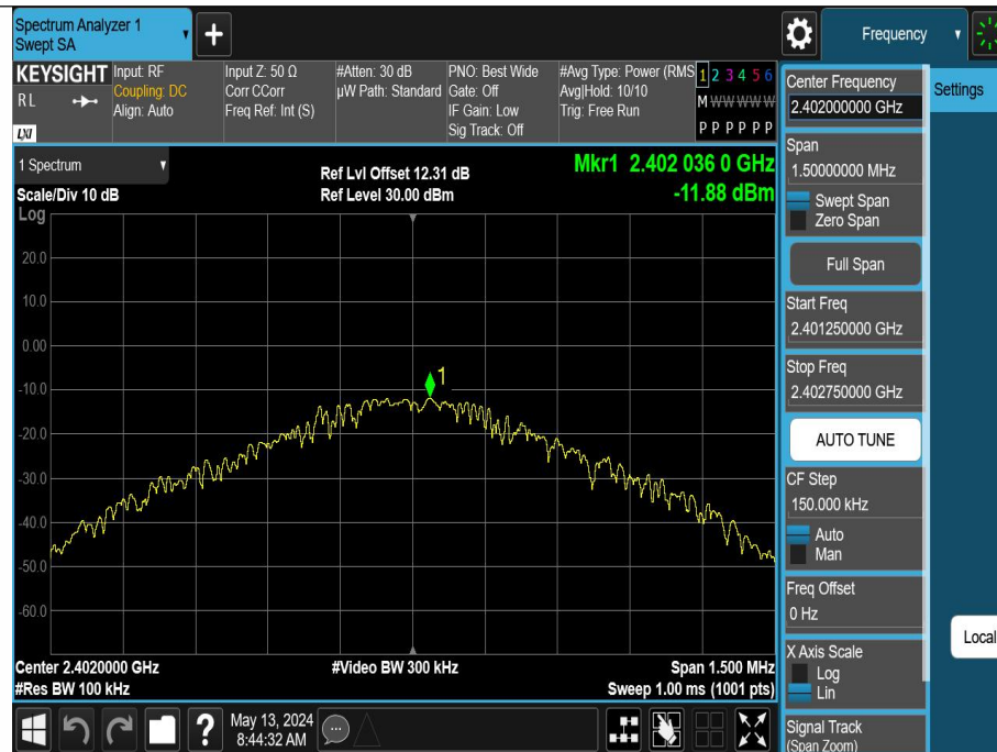
DH5-Ant1-2402-0~Reference-PASS
