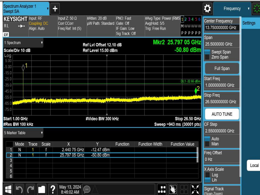
DH5-Ant1-2441-1000~26500-PASS
