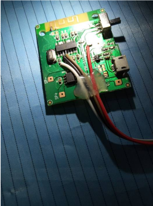
EUT – Main IC View 2
