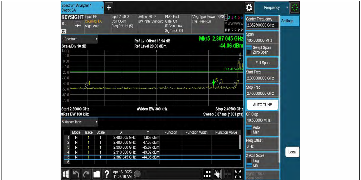
DH5-Ant1-Low-Hop_2402-1.86
