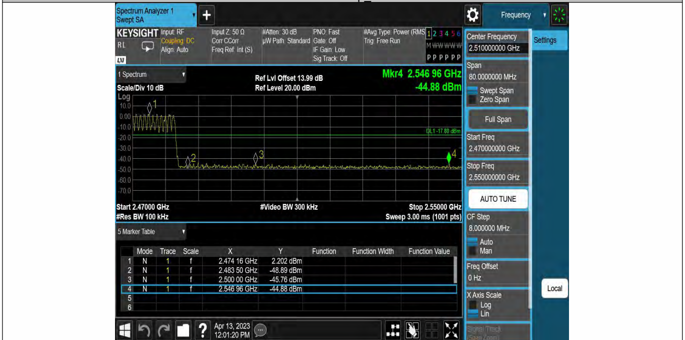
DH5-Ant1-High-Hop_2480-2.20
