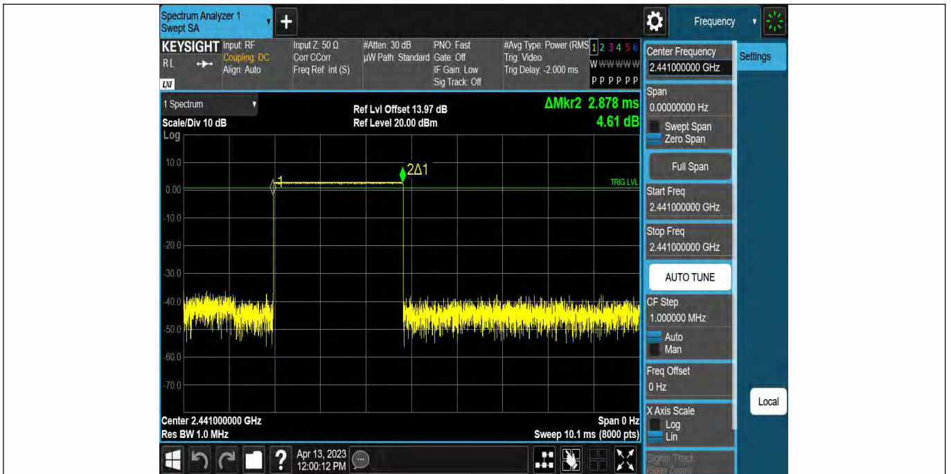
DH5-Ant1-Hop-2.878-106.67
