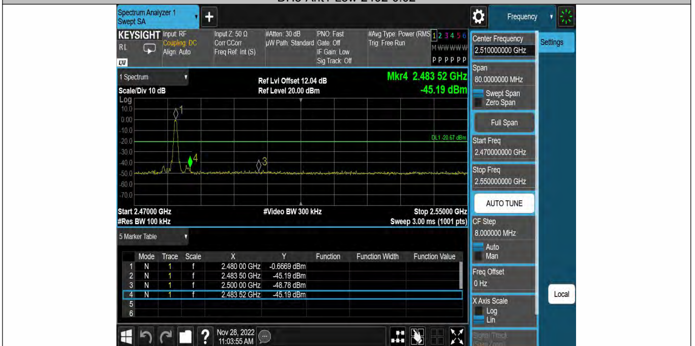
DH5-Ant1-High-2480-0.67
