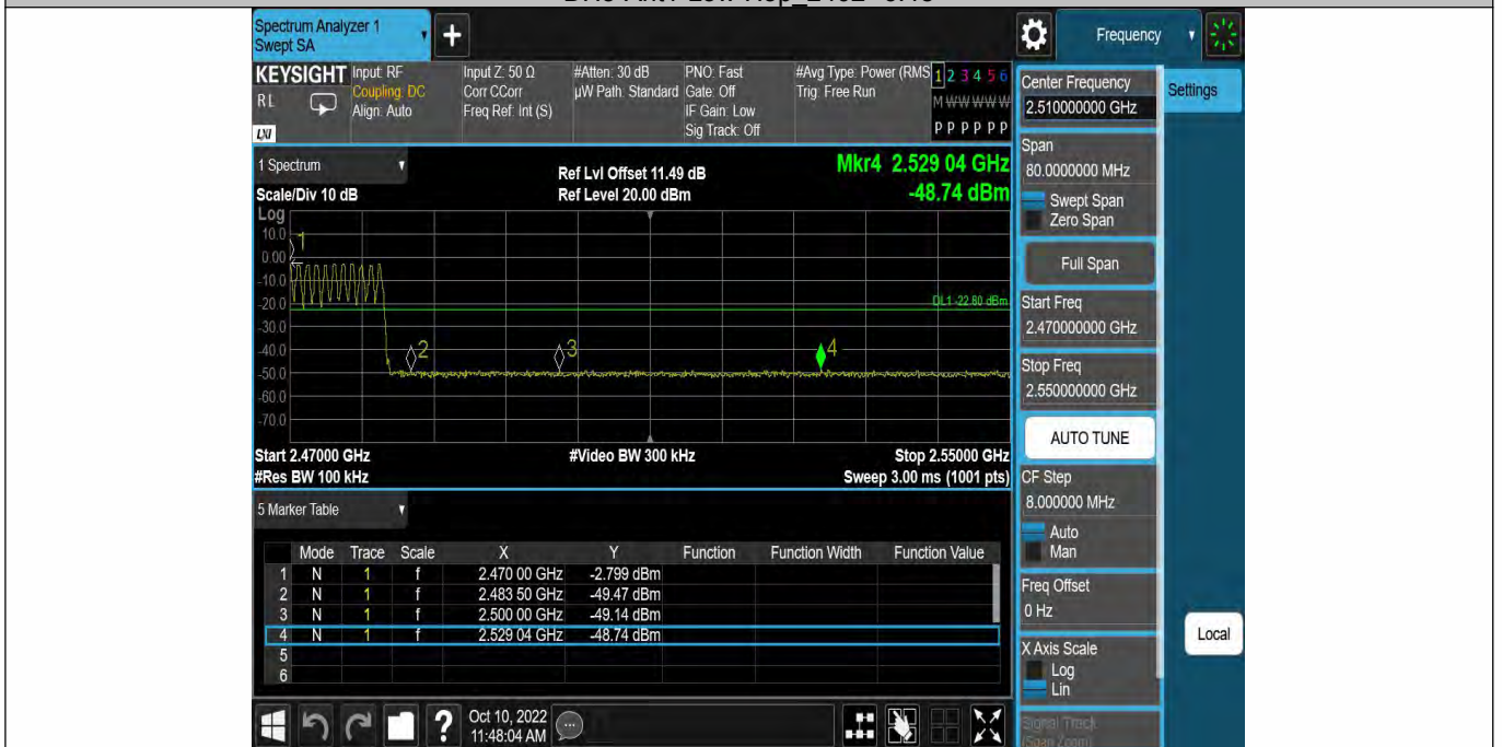
DH5-Ant1-High-Hop_2480--2.80
