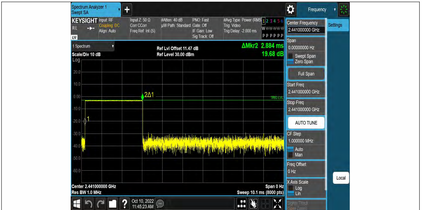
DH5-Ant1-Hop-2.884-106.67
