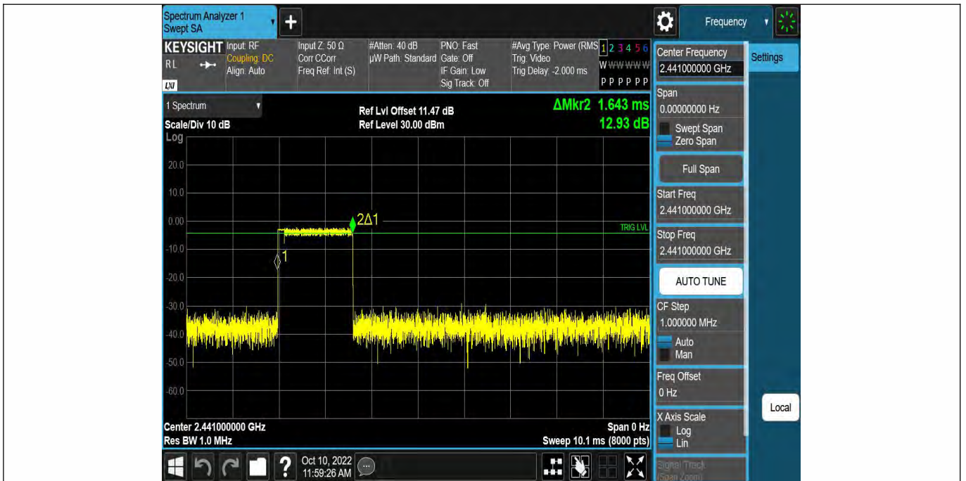
2DH3-Ant1-Hop-1.643-160
