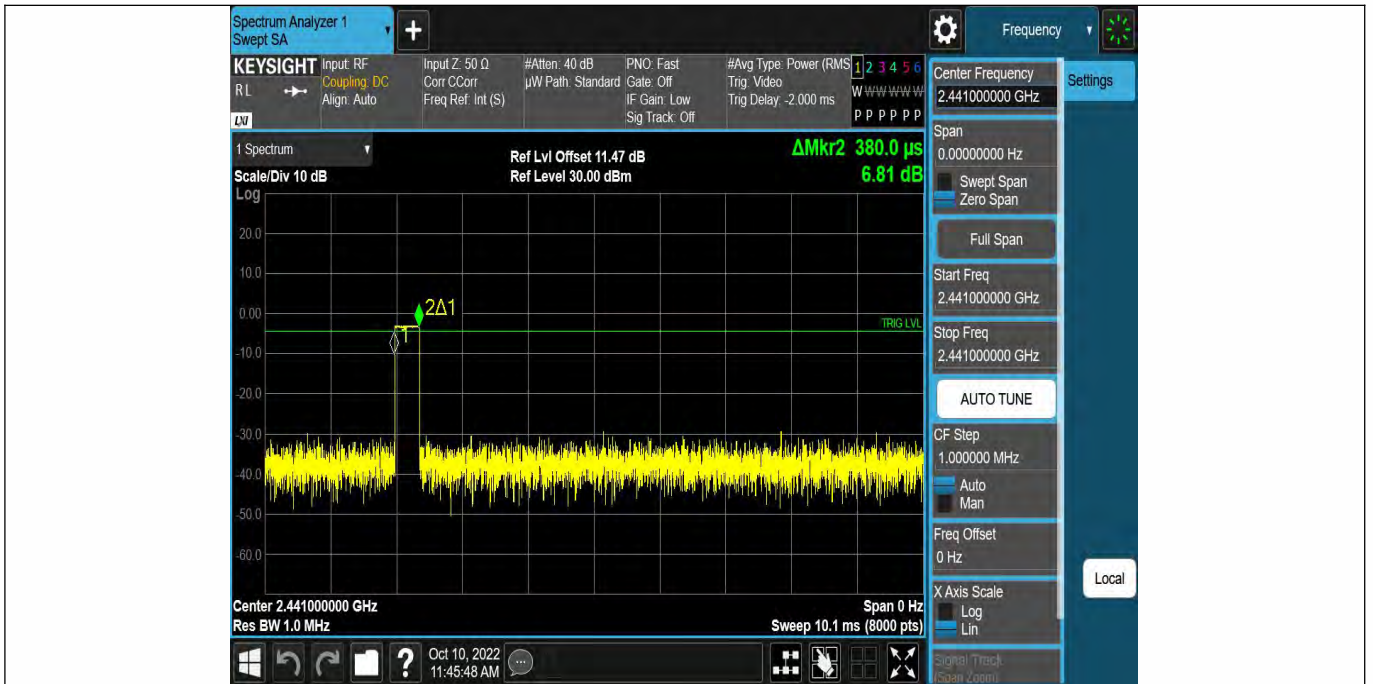
DH1-Ant1-Hop-0.380-320
