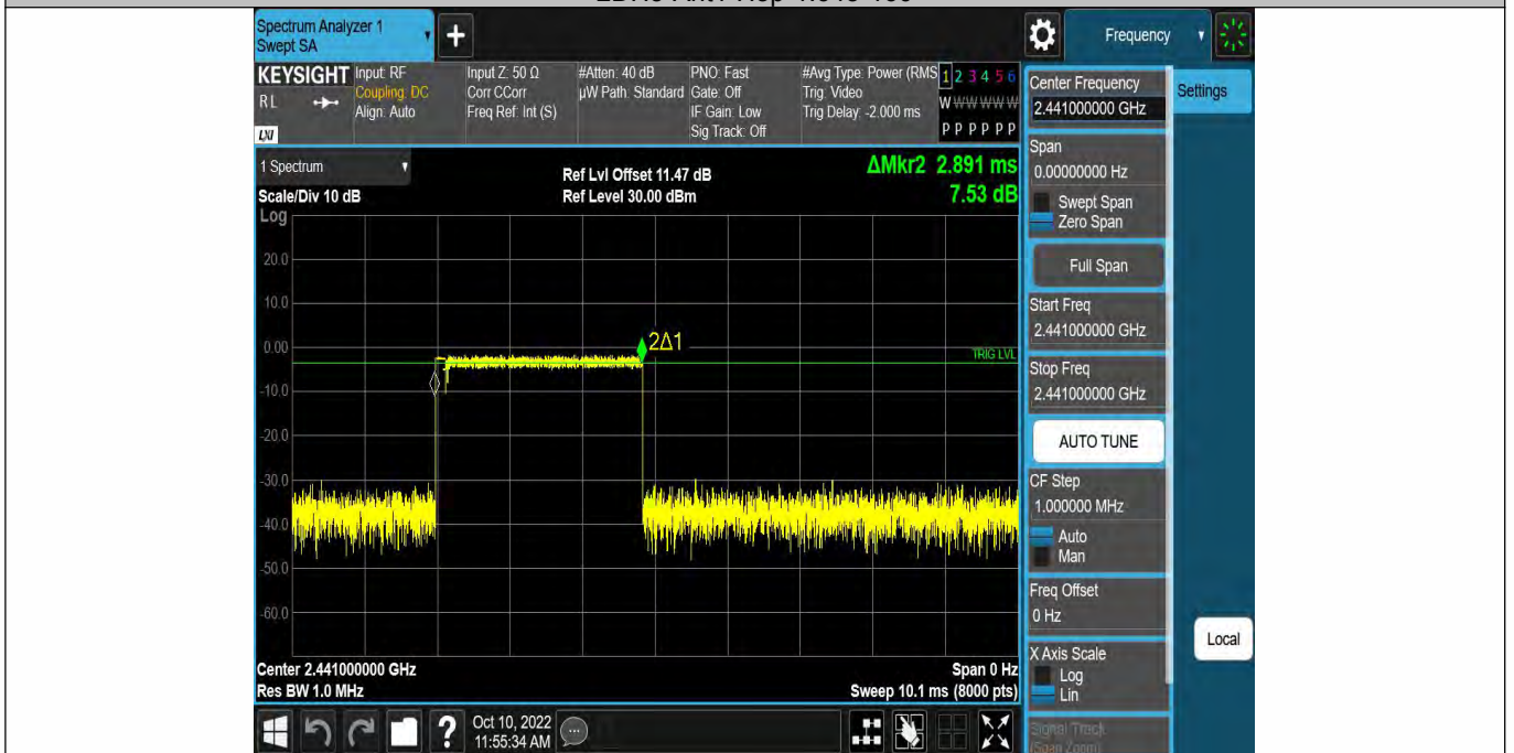
2DH5-Ant1-Hop-2.891-106.67
