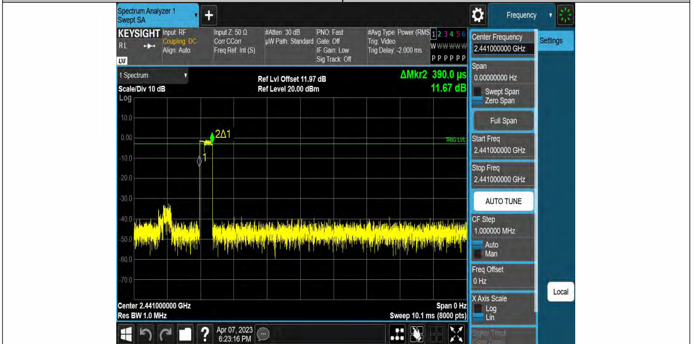
2DH1-Ant1-Hop-0.390-320
