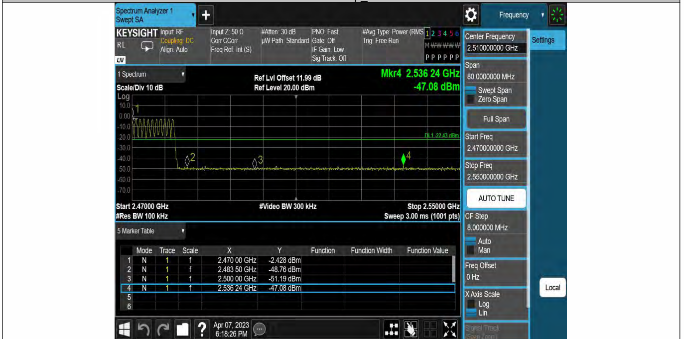
DH5-Ant1-High-Hop_2480--2.43
