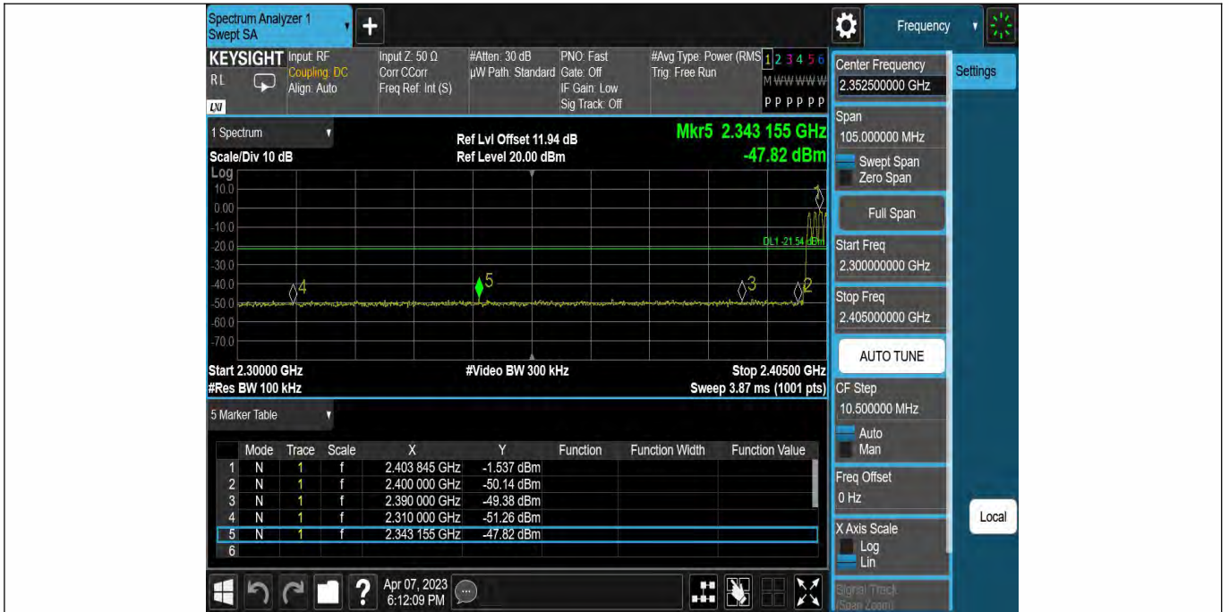
DH5-Ant1-Low-Hop_2402--1.54
