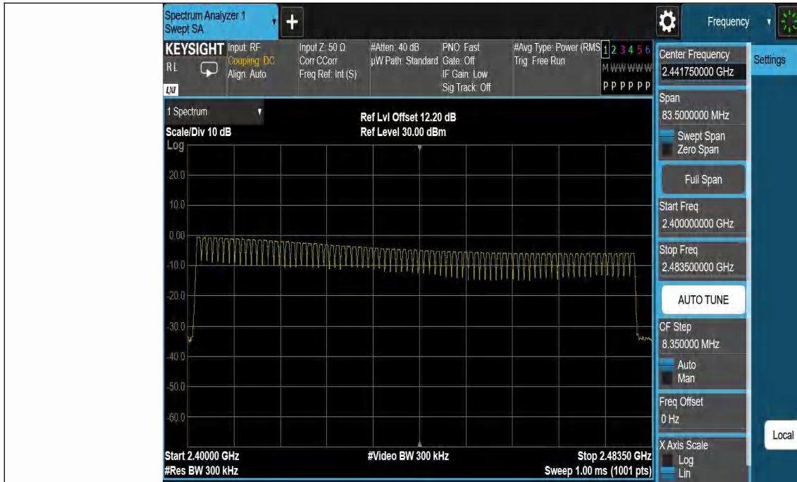
DH5-Ant1-Hop-PASS
