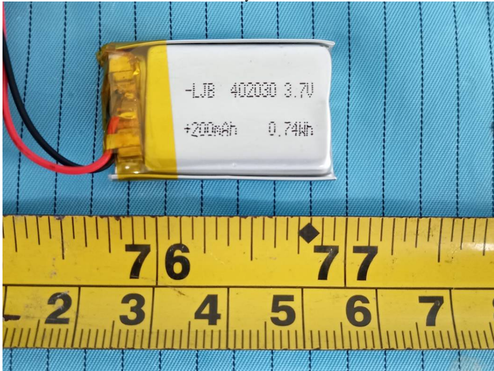
Battery Label
