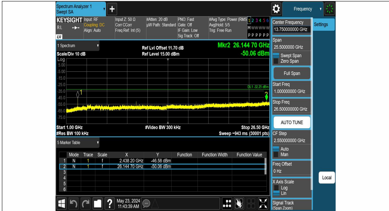
BLE_2M-Ant1-2440-1000~26500-PASS
