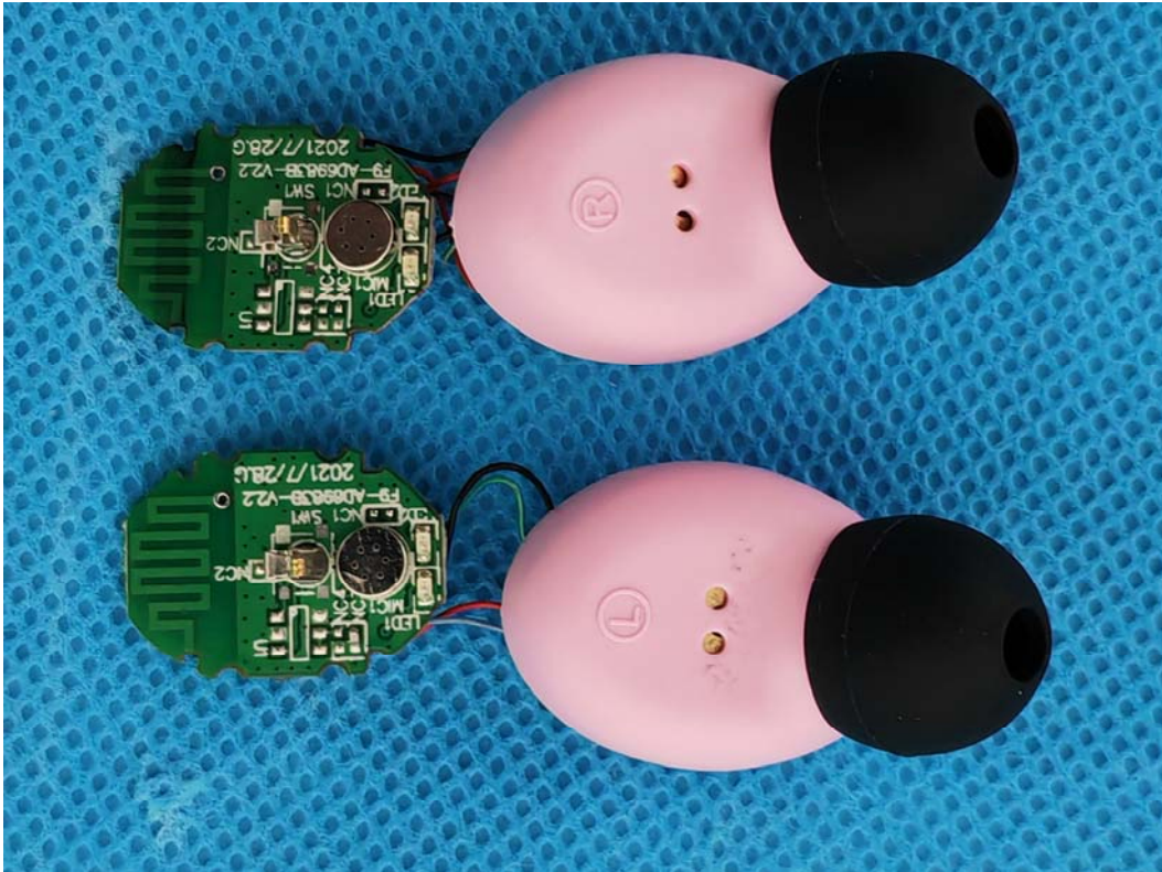
left earbud have one resistance without functional to distinguish left earbud and right earbud
