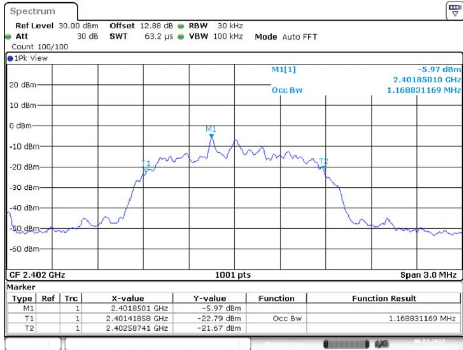
2DH1_Ant1_2402
