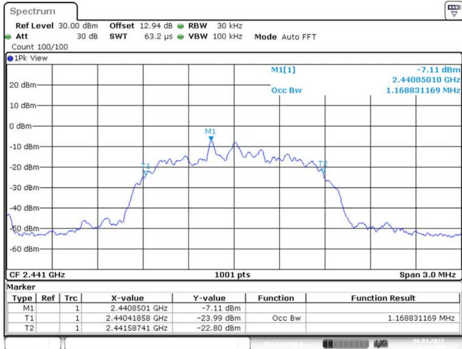
2DH1_Ant1_2441
