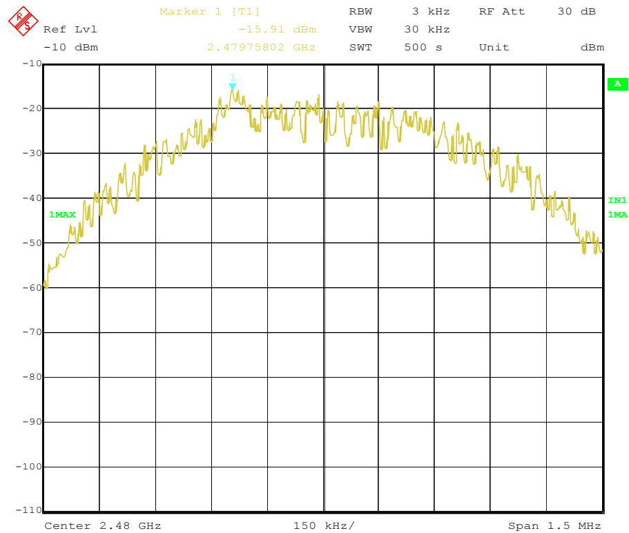
Di Figure 11 Peak Power Spectral Density(Higher ch_2480.000MHz)
