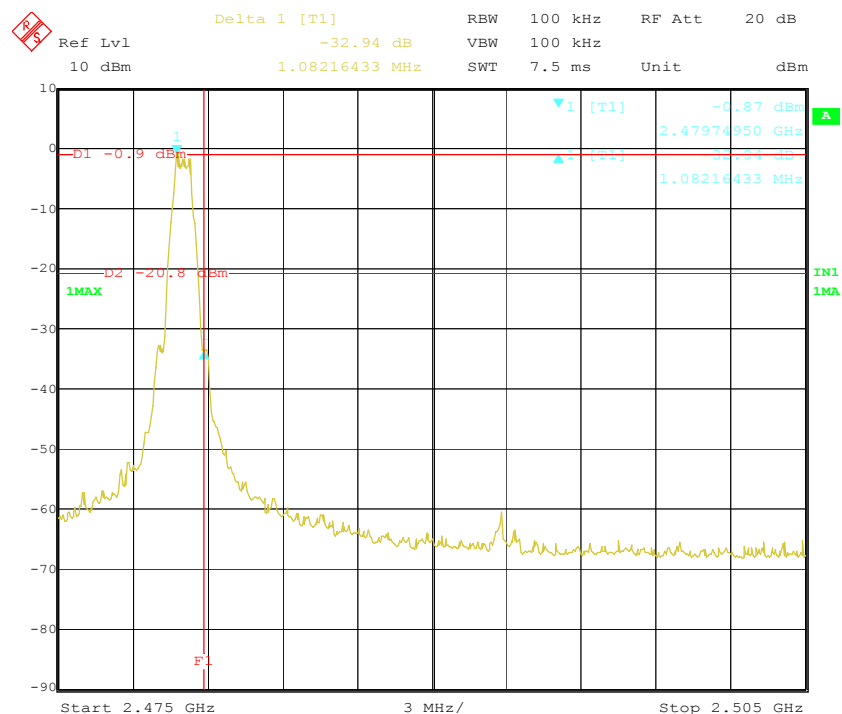
Figure 8 High Band Edge Plot on Channel 39_2480.000MHz
