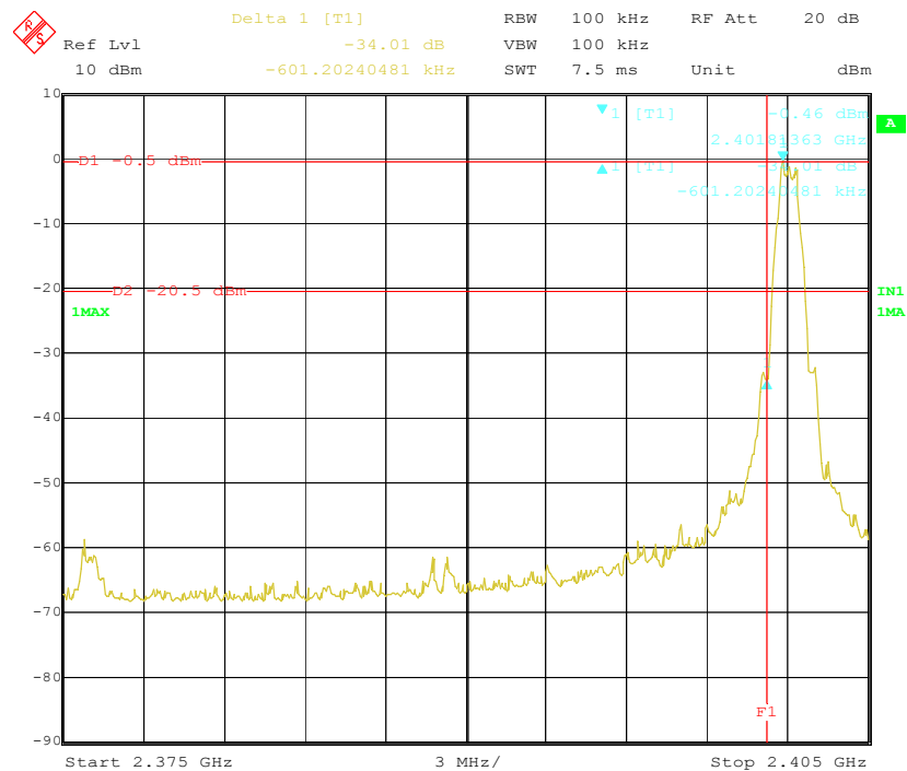
Figure 7 Low Band Edge Plot on Channel 00_2402.000MHz
