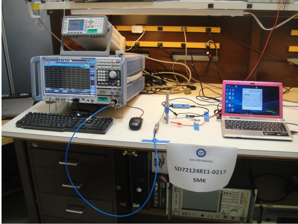
Temporary Antenna Port Measurement
