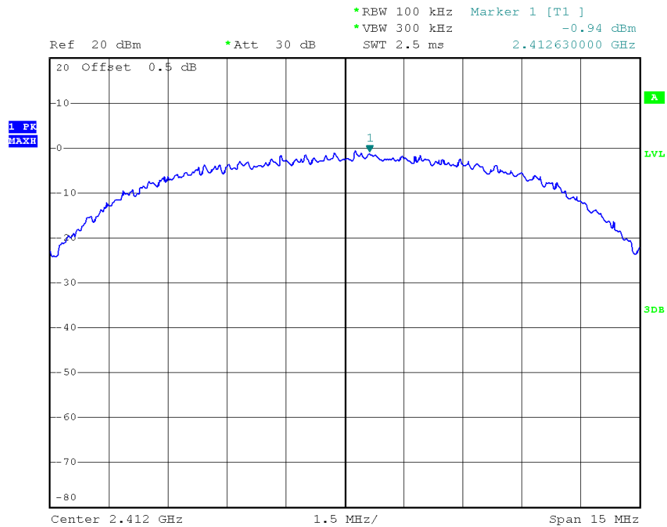
802.11b - PSD Plot on Channel 1
