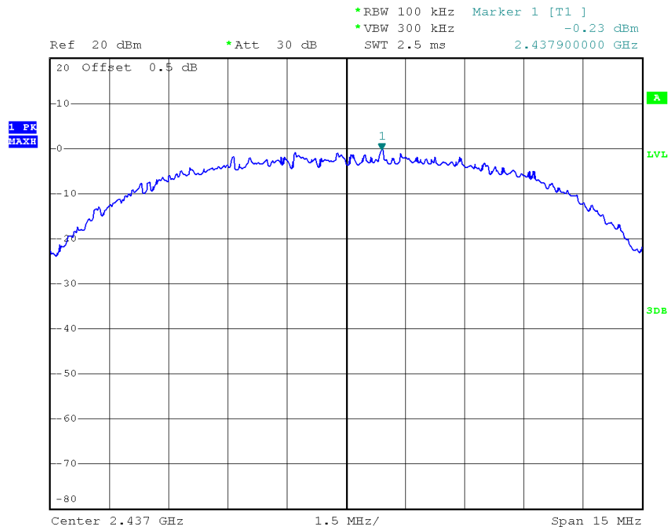
802.11b - PSD Plot on Channel 6
