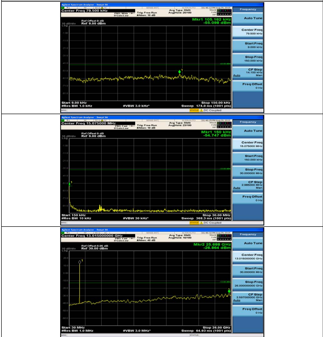
(Channel Bandwidth: 20 MHz)_MCH_QPSK_1RB#99
