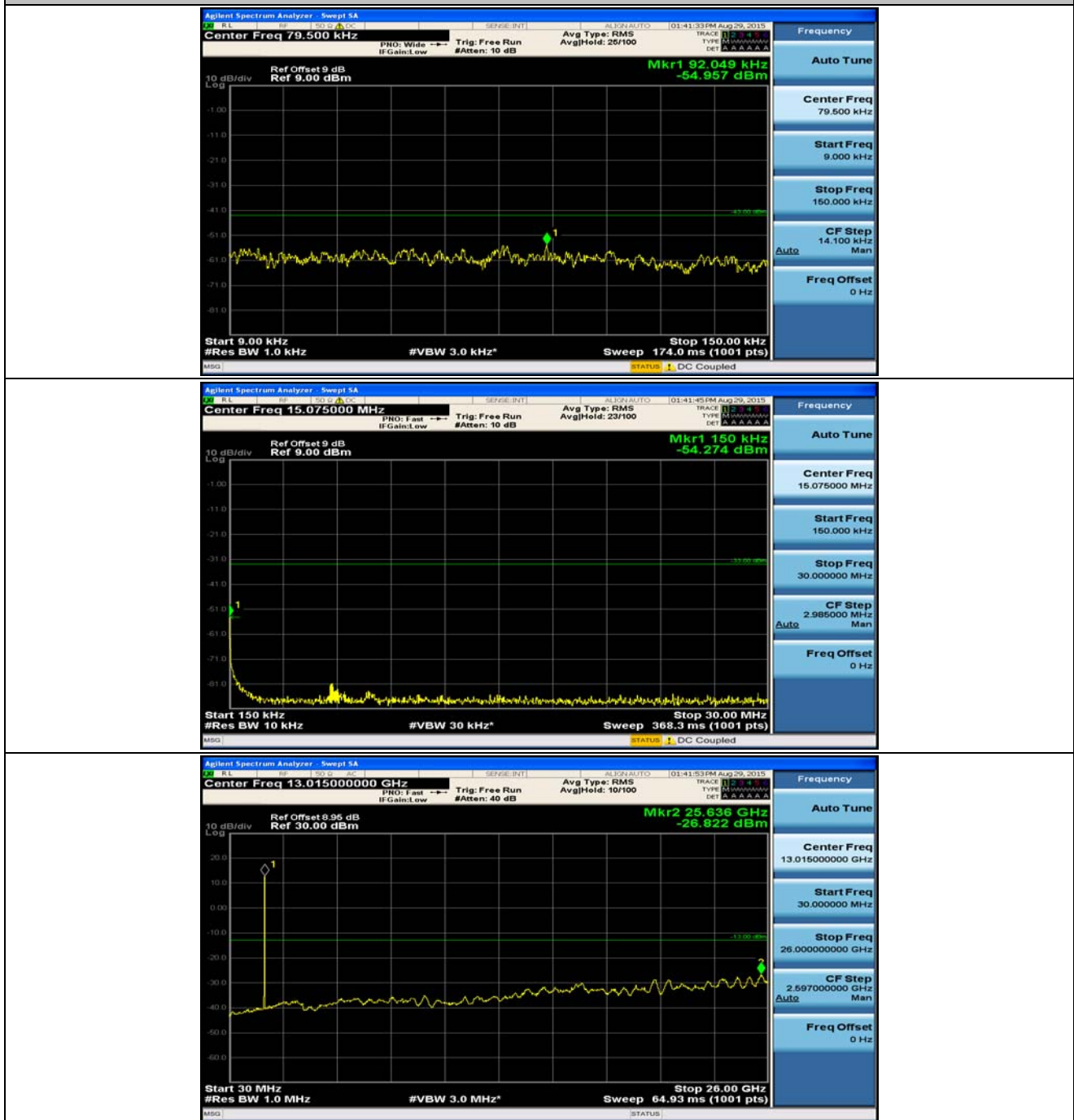
(Channel Bandwidth: 15 MHz)_HCH_16QAM_1RB#74
