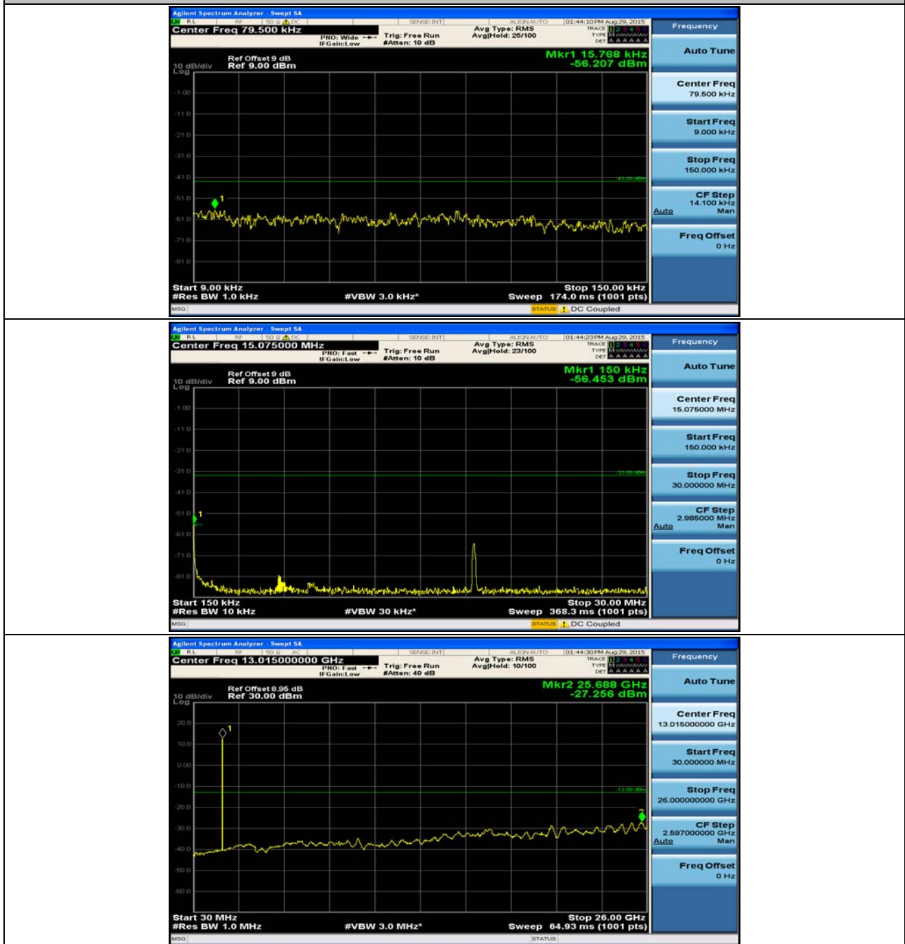
(Channel Bandwidth: 20 MHz)_LCH_16QAM_1RB#49
