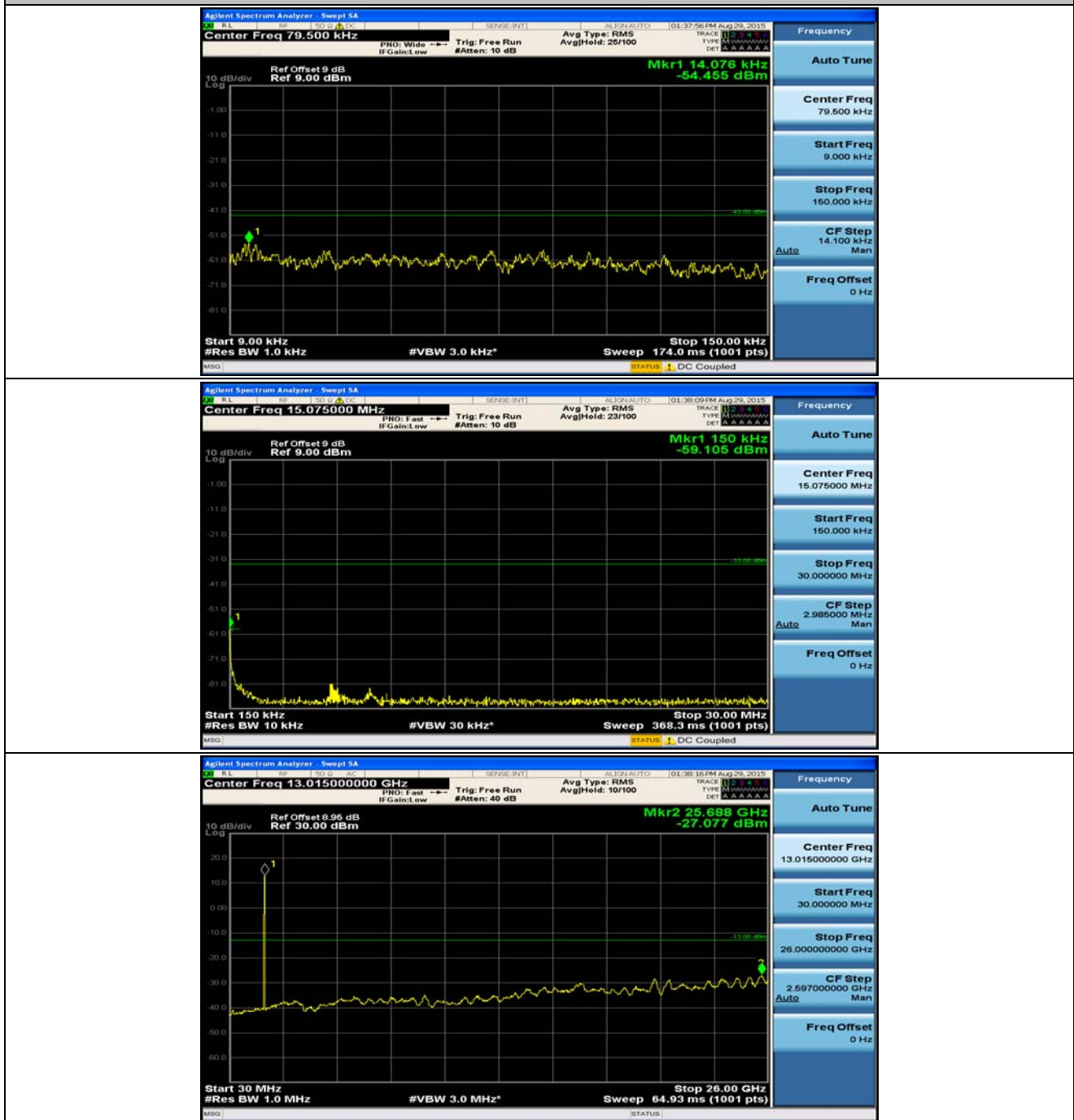
(Channel Bandwidth: 15 MHz)_MCH_16QAM_1RB#37
