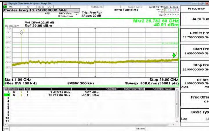
DH5_Ant1_2441_1000~26500
