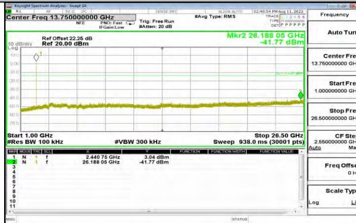
3DH5_Ant1_2441_1000~26500
