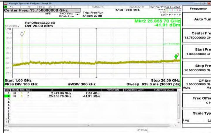
3DH5_Ant1_2480_1000~26500
