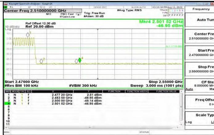
DH5_Ant1_High_Hop_2480
