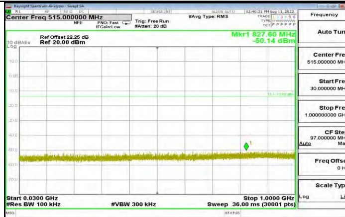
3DH5_Ant1_2441_30~1000
