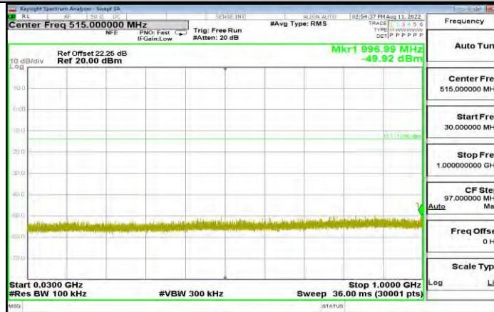
DH5_Ant1_2441_30~1000
