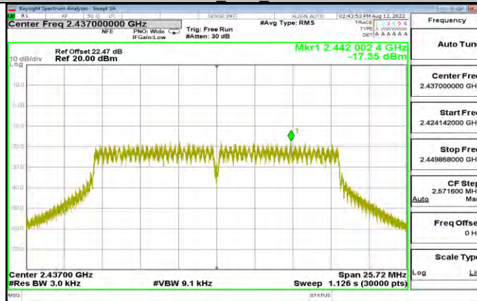
11G Ant1_2437
