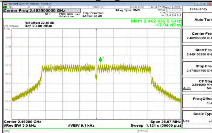
11G Ant1_2462
