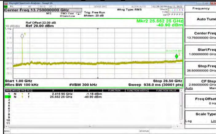
11G Ant1_2412_1000~26500
