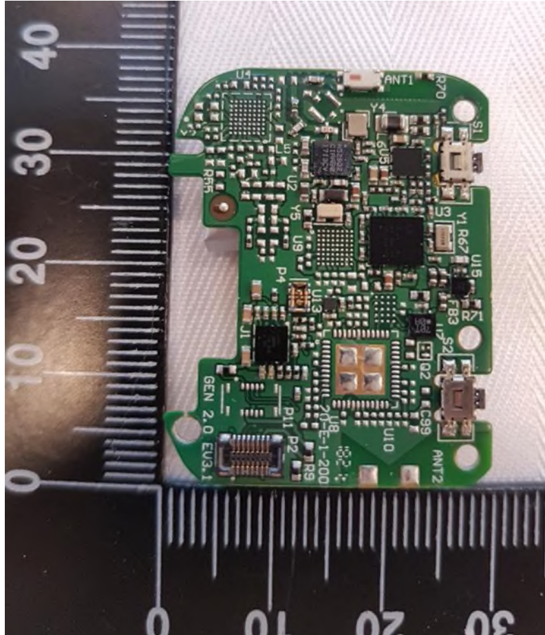
Figure 2 – EUT Internal Photo Front (MicroUSB connection removed)
