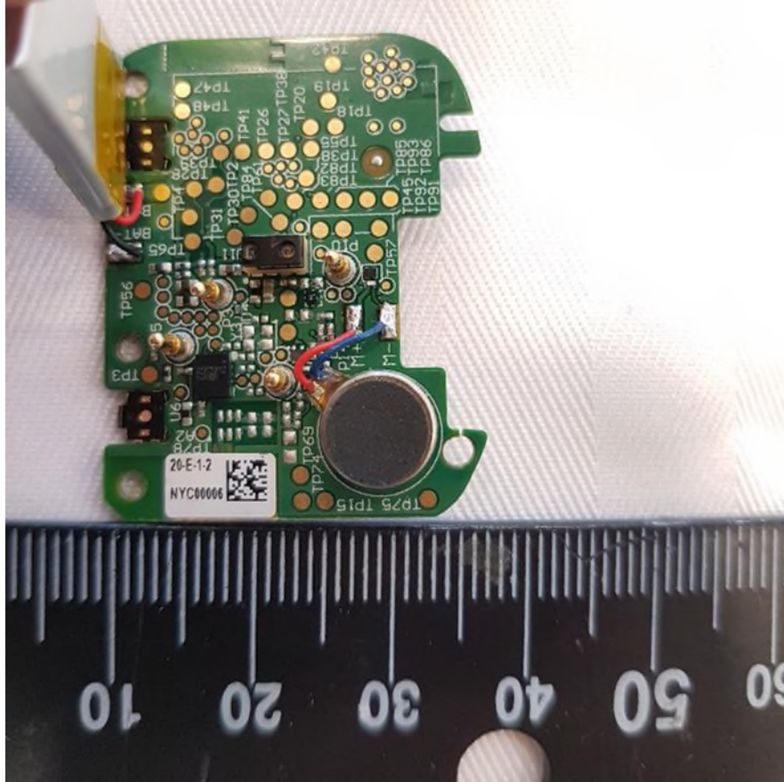
Figure 4 – EUT Internal Photo Back
