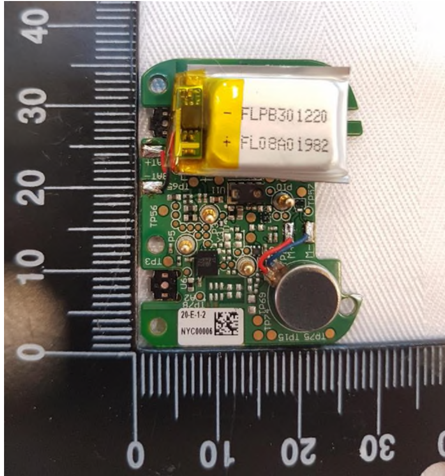
Figure 3 – EUT Internal Photo Back
