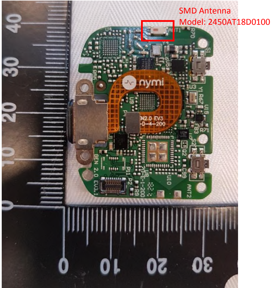
Figure 1 – EUT Internal Photo Front
