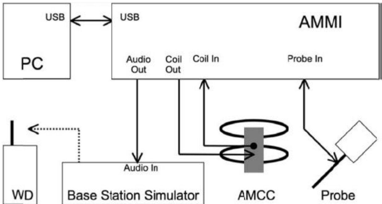
T-Coil setup with HAC Test Arch and AMCC
