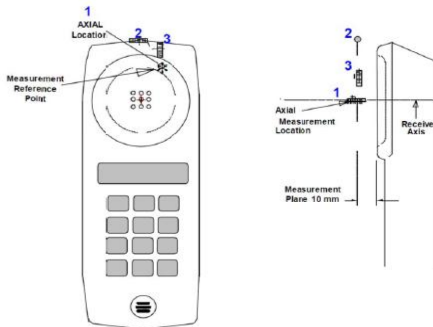
A typical DUT reference and plane for T-Coil measurement
