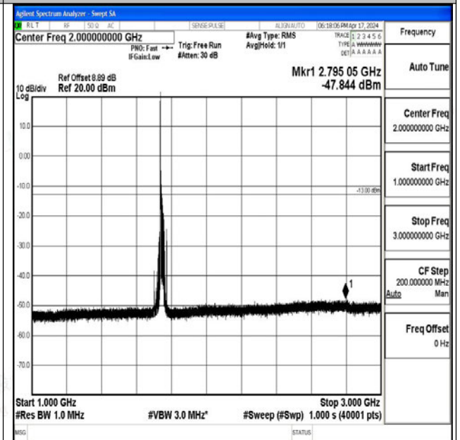
Band66_20MHz_QPSK_132322_1RB#0_1000~3000_1000~3000
