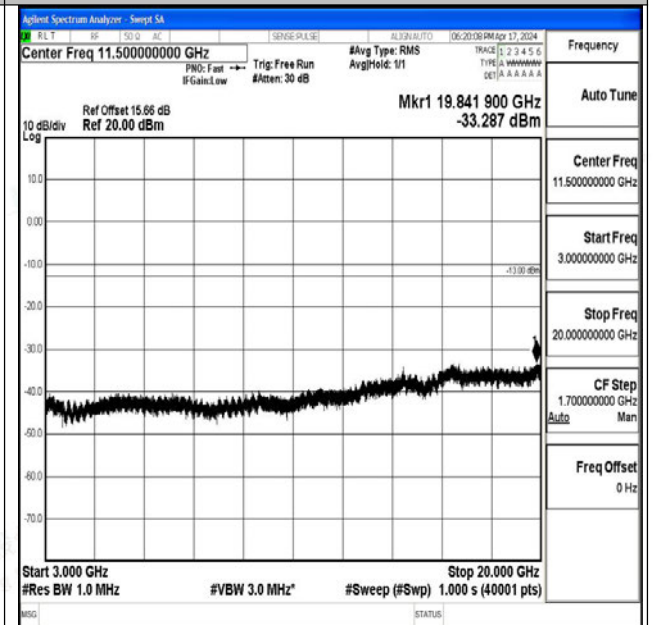
Band66_20MHz_16QAM_132572_1RB#0_3000~20000_3000~20000
