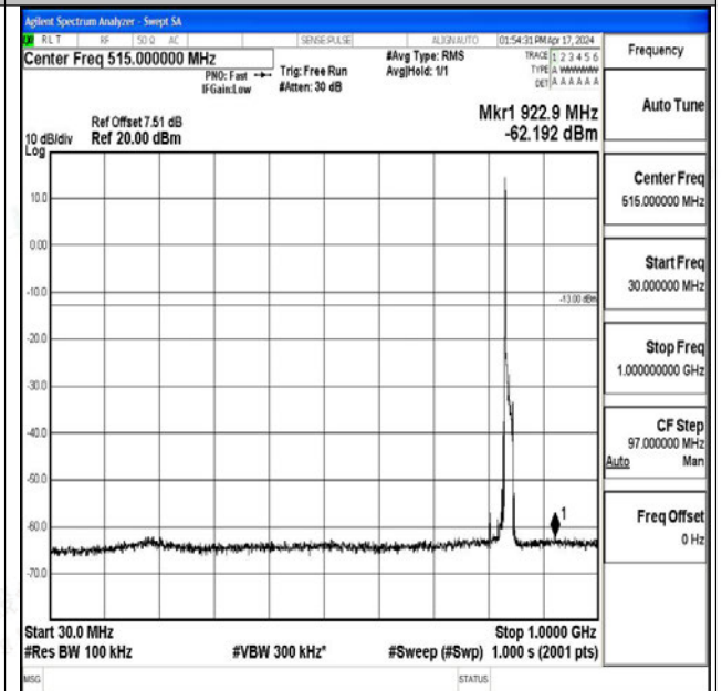
Band26_15MHz_16QAM_26965_1RB#0_30~1000_30~1 000
