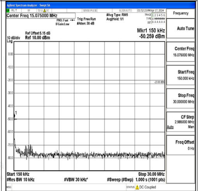
Band26_15MHz_QPSK_26915_1RB#0_0.15~30_0.15~3
