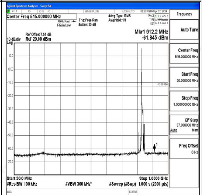
Band26_10MHz_16QAM_26915_1RB#0_30~1000_30~1 000
