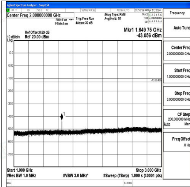
Band26_15MHz_16QAM_26865_1RB#0_1000~3000_10
