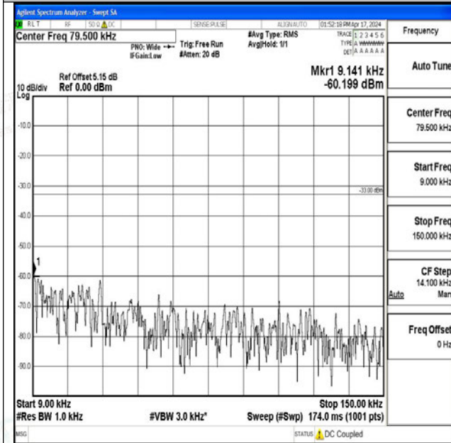
Band26_15MHz_QPSK_26915_1RB#0_0.009~0.15_0.00
