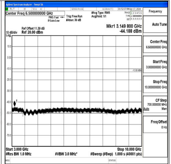
Band26_15MHz_16QAM_26865_1RB#0_3000~10000_3
