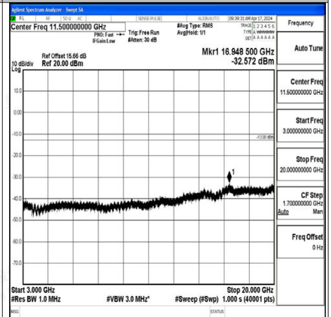
Band25_5MHz_16QAM_26365_1RB#0_3000~20000_30
