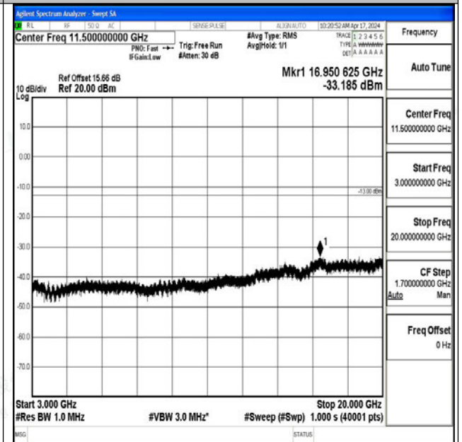
Band25_15MHz_16QAM_26365_1RB#0_3000~20000_3000~20000
