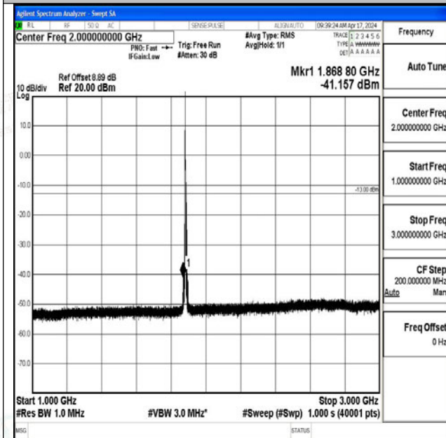
Band25_5MHz_16QAM_26365_1RB#0_1000~3000_100
