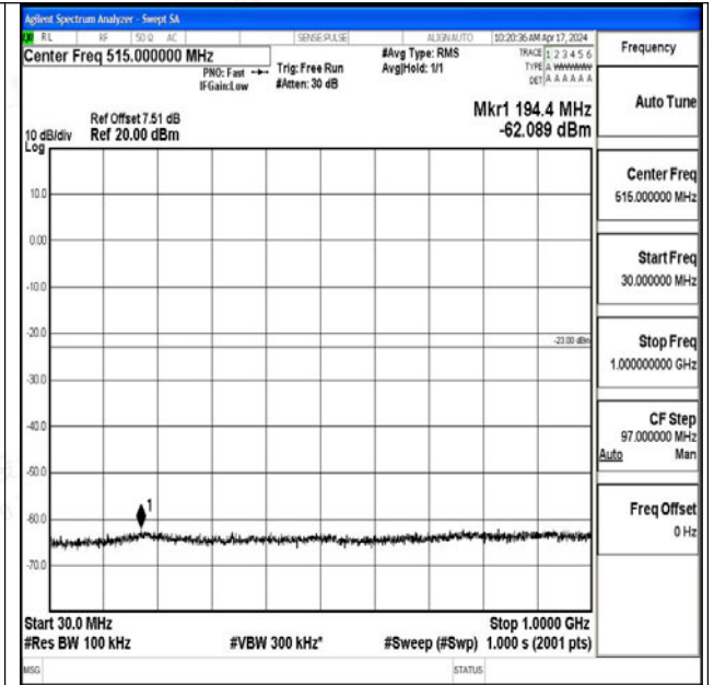
Band25_15MHz_16QAM_26365_1RB#0_30~1000_30~1000
