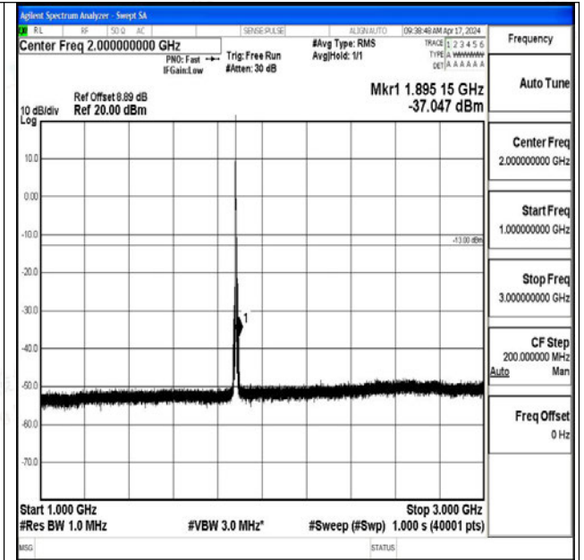
Band25_5MHz_QPSK_26365_1RB#0_1000~3000_1000~3000
