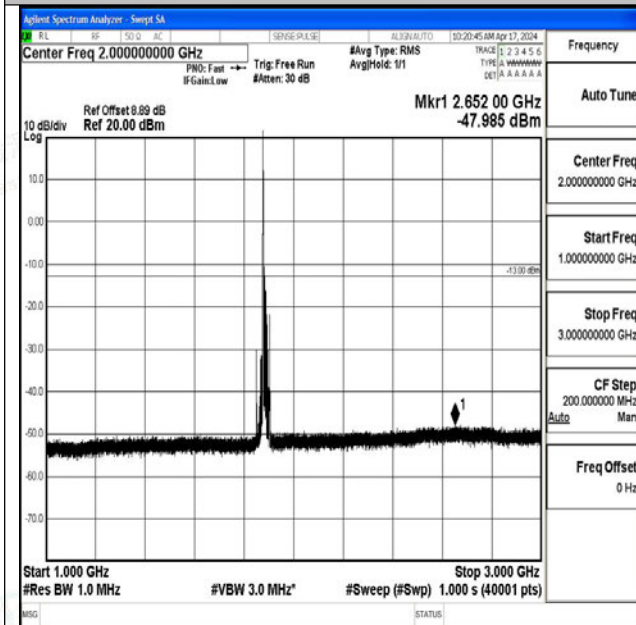
Band25_15MHz_16QAM_26365_1RB#0_1000~3000_1000~3000
