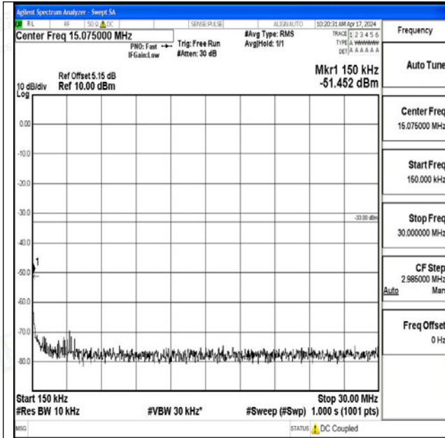
Band25_15MHz_16QAM_26365_1RB#0_0.15~30_0.15~30
