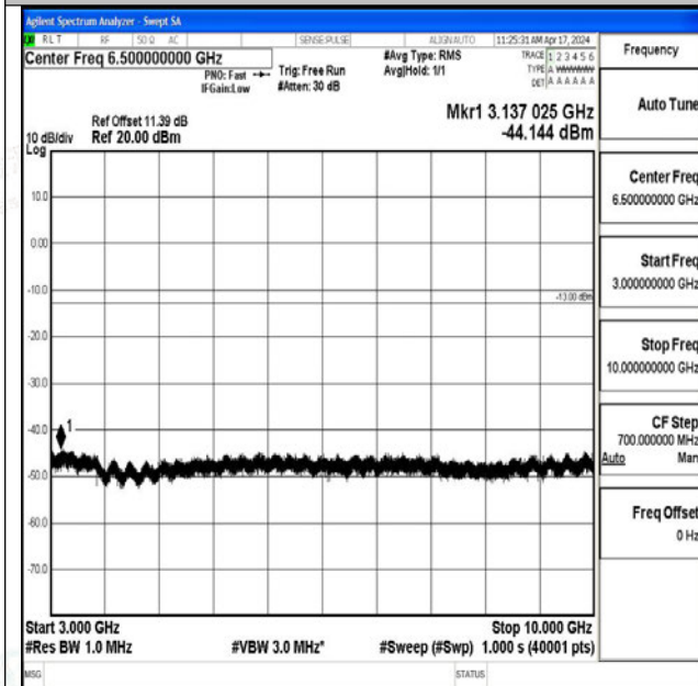
Band26_3MHz_QPSK_26705_1RB#0_3000~10000_300~10000
