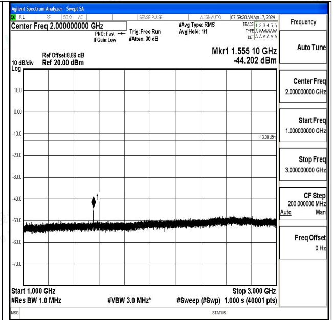
Band13_10MHz_QPSK_23230_1RB#0_1000~3000_100
