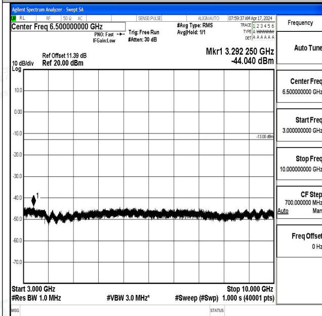
Band13_10MHz_QPSK_23230_1RB#0_3000~10000_30
