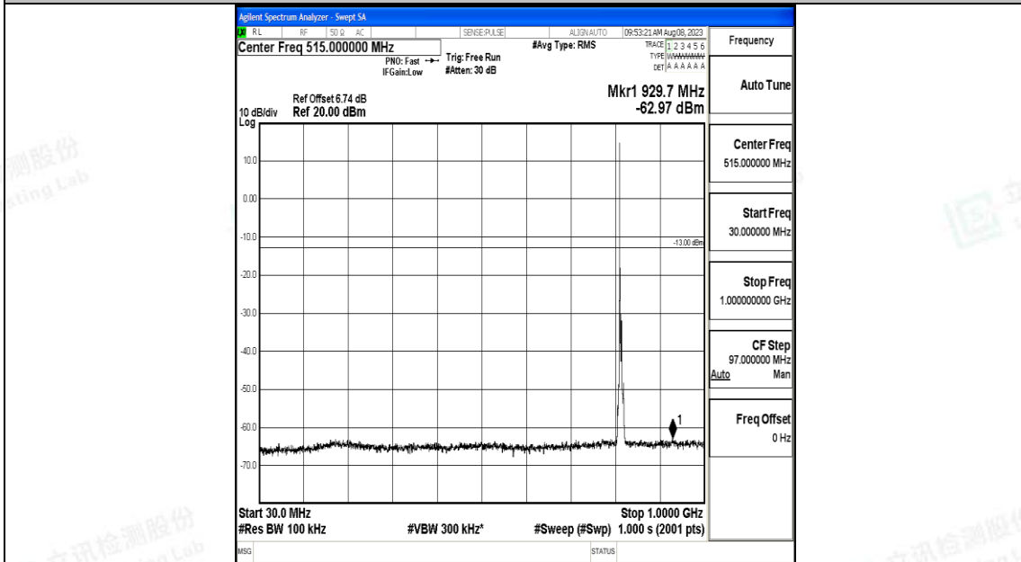
Band26_5MHz_16QAM_26715_1RB#0_30~1000_30~1000
