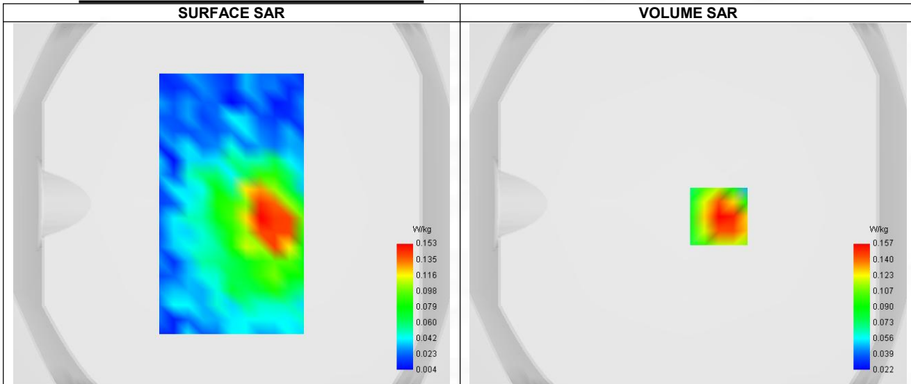
Maximum location: X=17.00, Y=-7.00 ; SAR Peak: 0.19 W/kg
