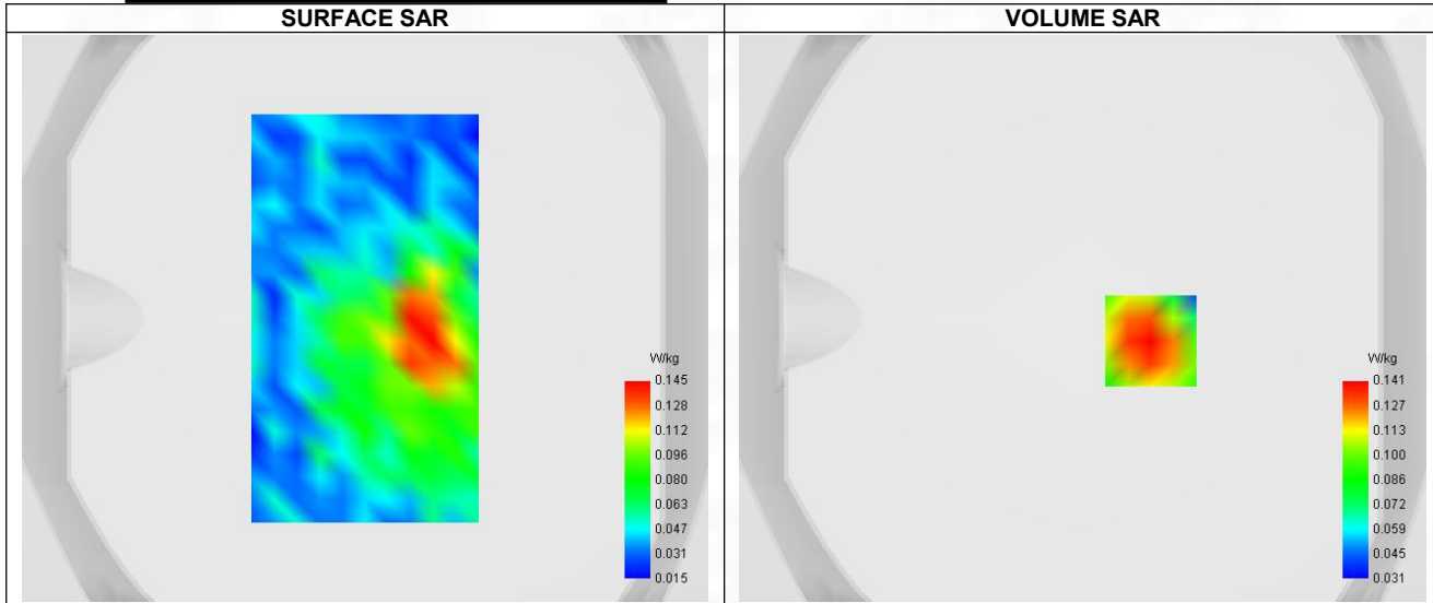
Maximum location: X=24.00, Y=-8.00 ; SAR Peak: 0.17 W/kg
