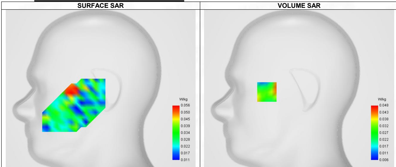
Maximum location: X=-53.00, Y=-6.00 ; SAR Peak: 0.09 W/kg
