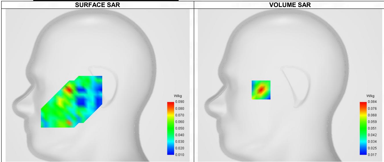
Maximum location: X=-49.00, Y=-8.00 ; SAR Peak: 0.11 W/kg
