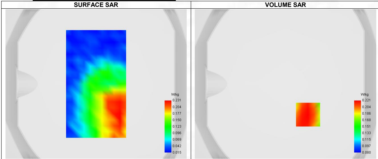
Maximum location: X=30.00, Y=-41.00 ; SAR Peak: 0.27 W/kg
