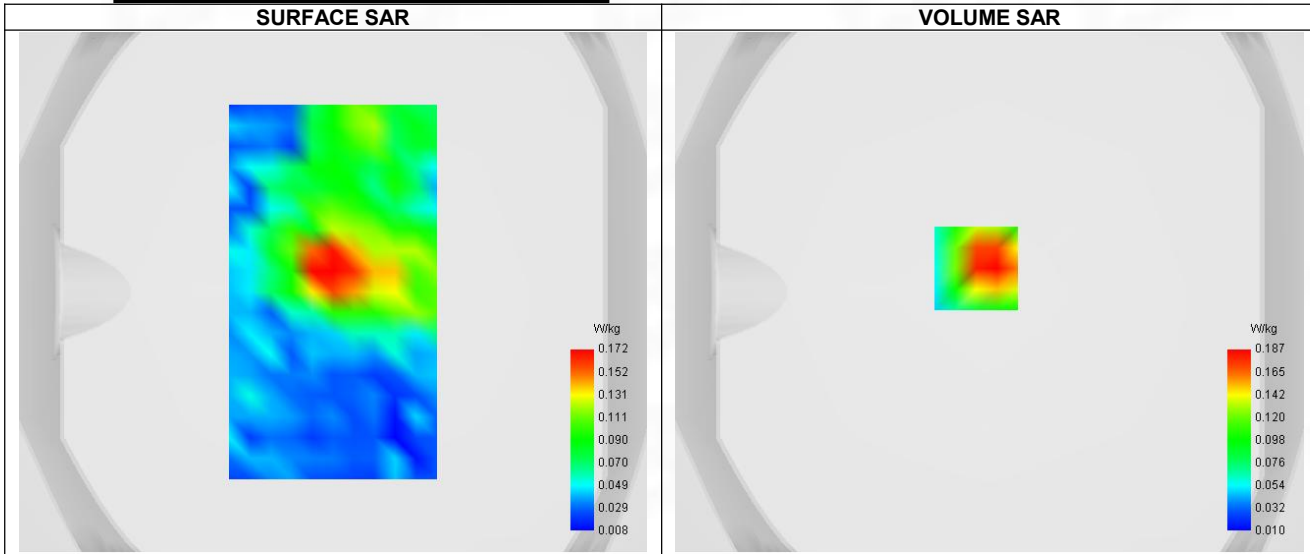
Maximum location: X=-5.00, Y=9.00 ; SAR Peak: 0.32 W/kg
