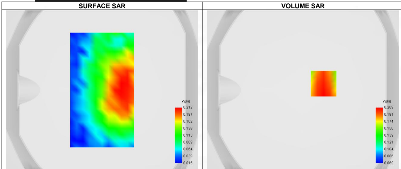
Maximum location: X=26.00, Y=8.00 ; SAR Peak: 0.25 W/kg
