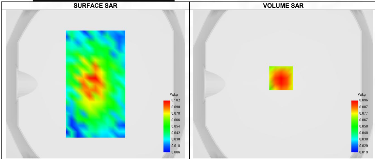
Maximum location: X=-32.00, Y=-48.00 ; SAR Peak: 0.12 W/kg
