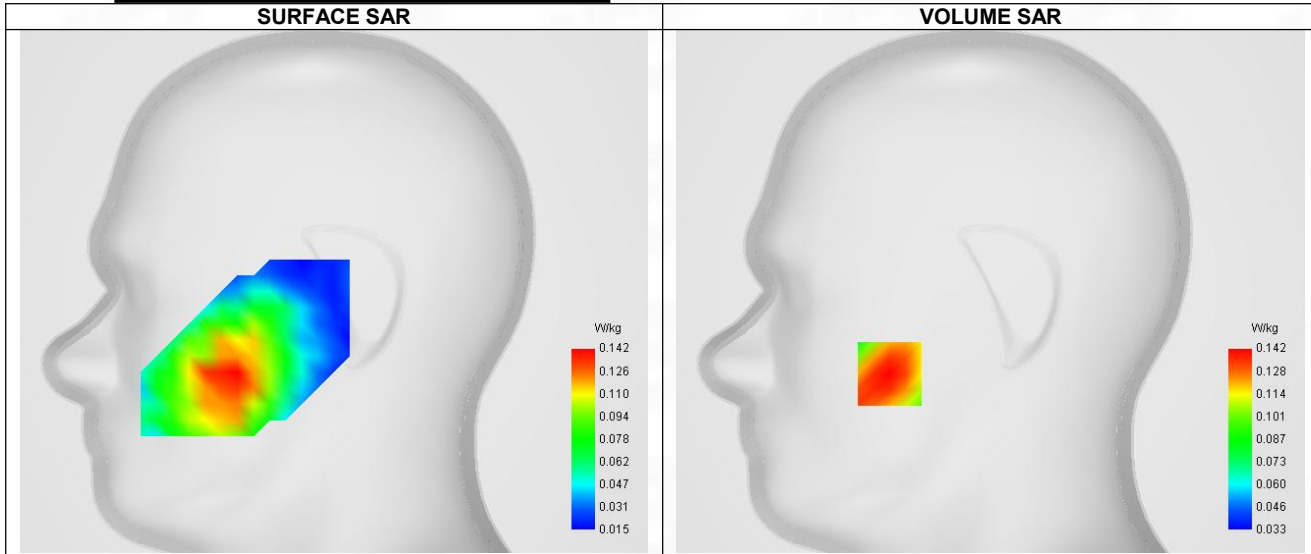
Maximum location: X=-50.00, Y=-41.00 ; SAR Peak: 0.18 W/kg
