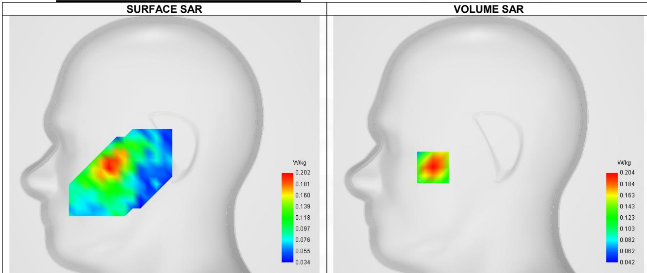
Maximum location: X=-56.00, Y=-23.00 ; SAR Peak: 0.29 W/kg
