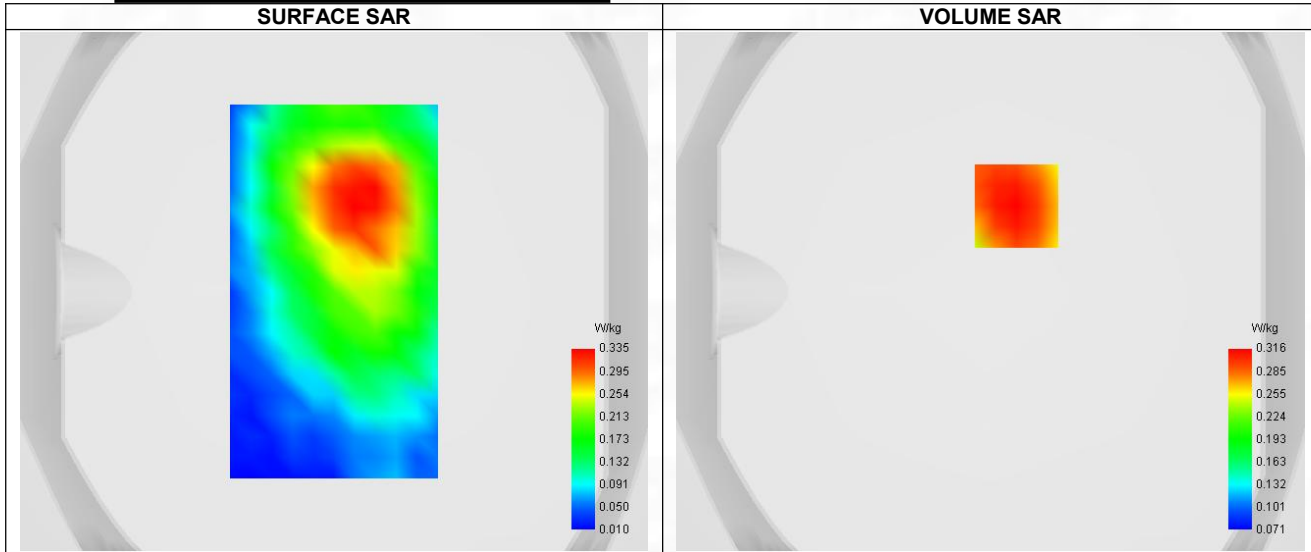
Maximum location: X=10.00, Y=33.00 ; SAR Peak: 0.39 W/kg
