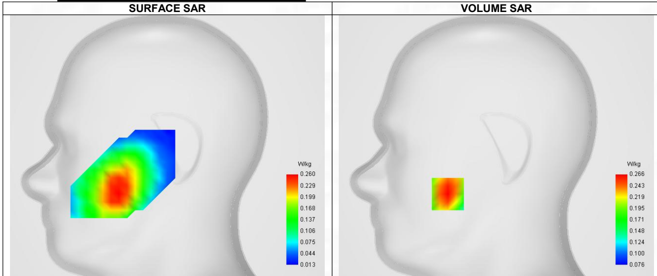
Maximum location: X=-48.00, Y=-48.00 ; SAR Peak: 0.33 W/kg
