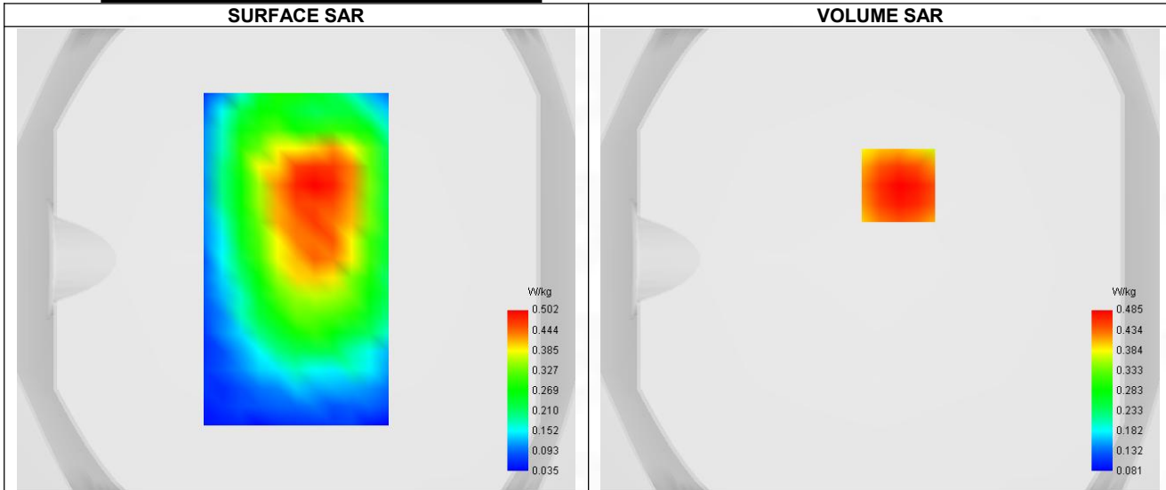
Maximum location: X=8.00, Y=32.00 ; SAR Peak: 0.58 W/kg
