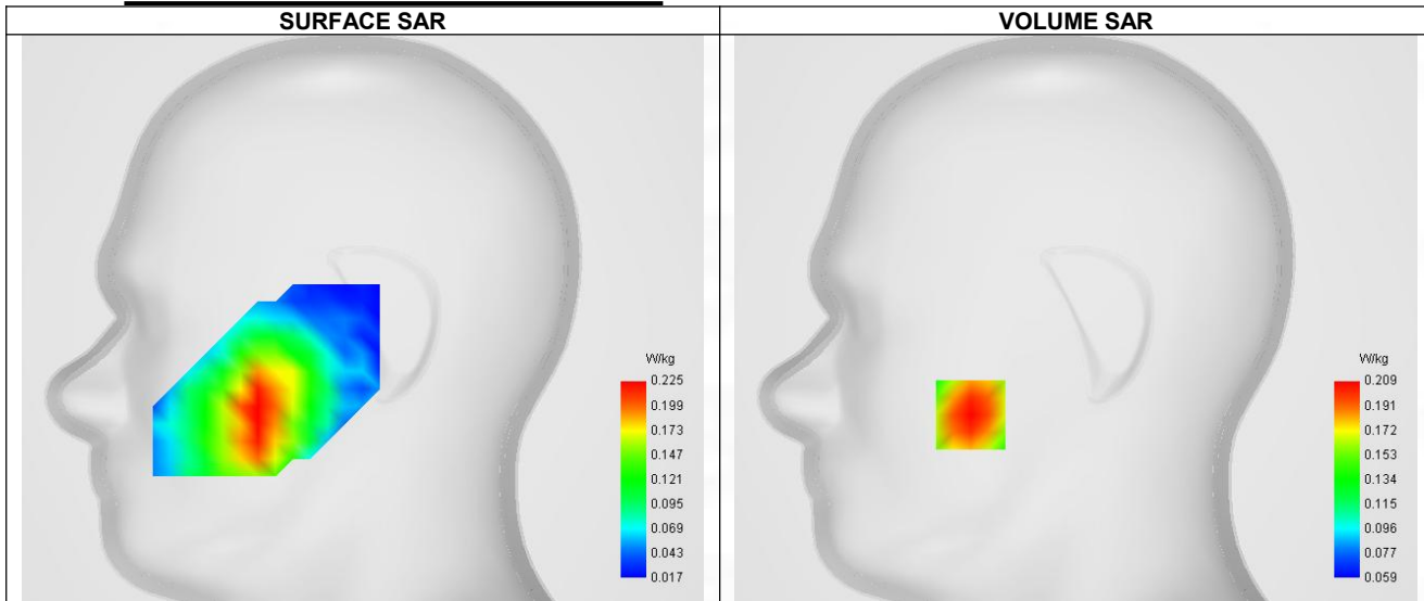
Maximum location: X=-48.00, Y=-44.00 ; SAR Peak: 0.24 W/kg
