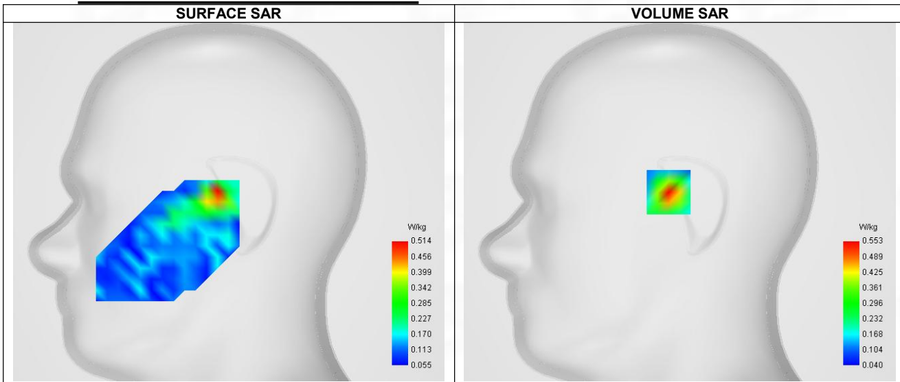
Maximum location: X=-8.00, Y=7.00 ; SAR Peak: 1.41 W/kg
