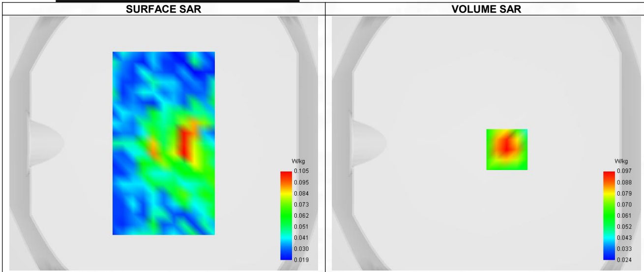
Maximum location: X=16.00, Y=-5.00 ; SAR Peak: 0.12 W/kg
