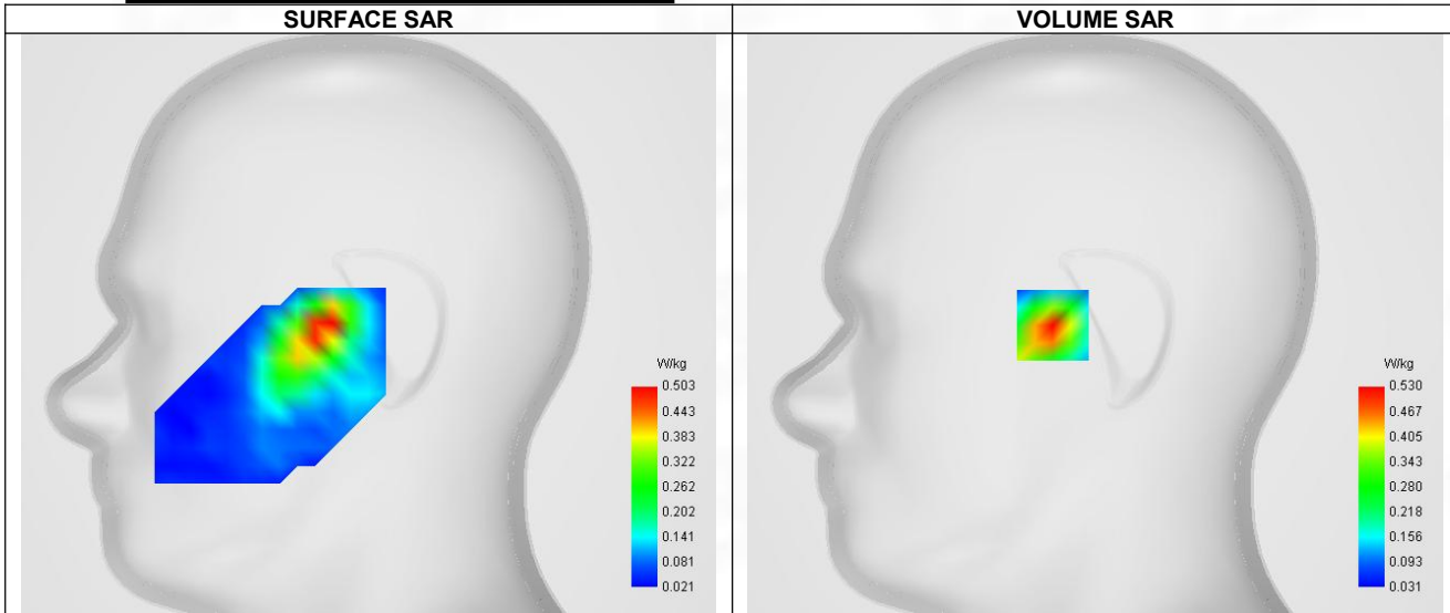
Maximum location: X=-19.00, Y=-1.00 ; SAR Peak: 0.90 W/kg
