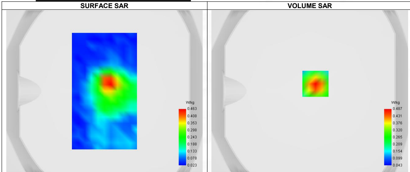
Maximum location: X=7.00, Y=9.00 ; SAR Peak: 0.79 W/kg
