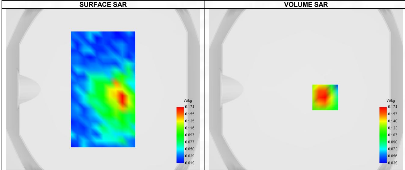
Maximum location: X=24.00, Y=-10.00 ; SAR Peak: 0.24 W/kg
