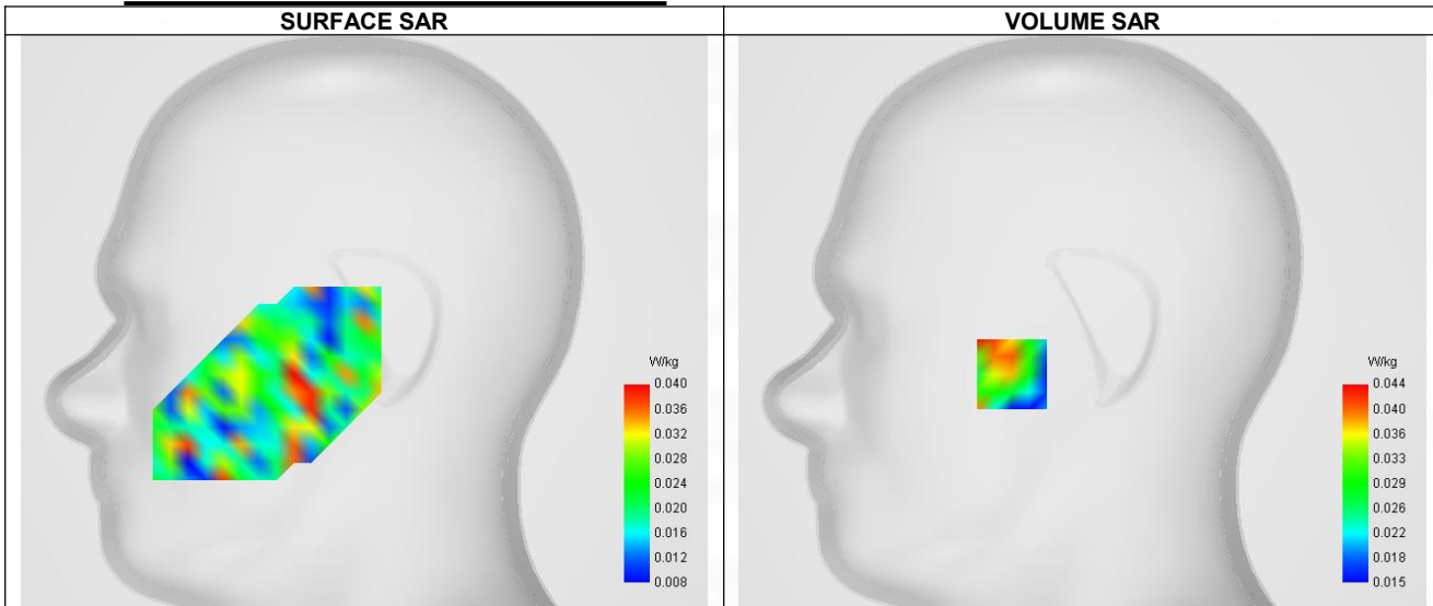
Maximum location: X=-32.00, Y=-24.00 ; SAR Peak: 0.07 W/kg
