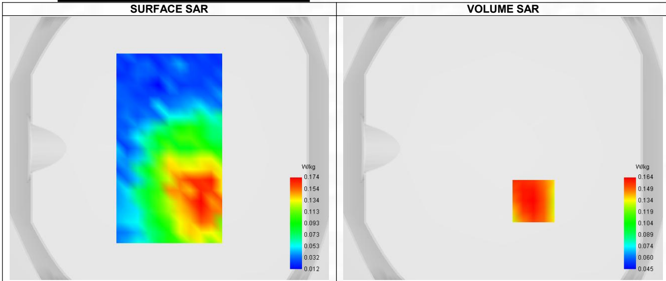
Maximum location: X=23.00, Y=-40.00 ; SAR Peak: 0.21 W/kg
