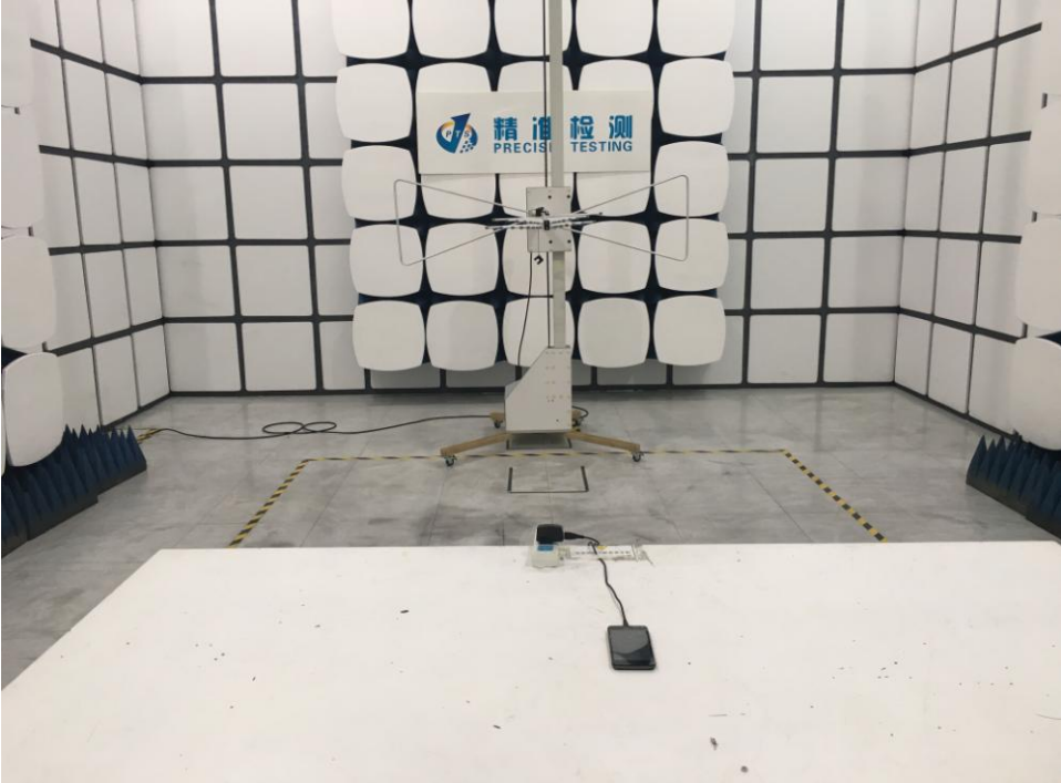
FCC RADIATED EMISSION TEST SETUP
