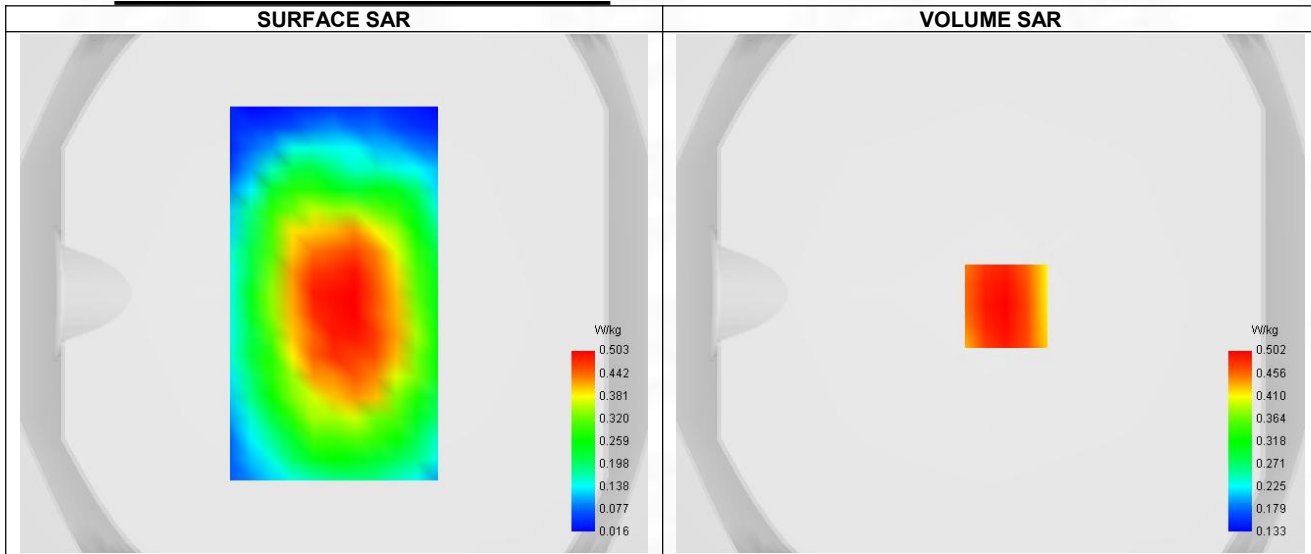
Maximum location: X=6.00, Y=-5.00 ; SAR Peak: 0.62 W/kg
