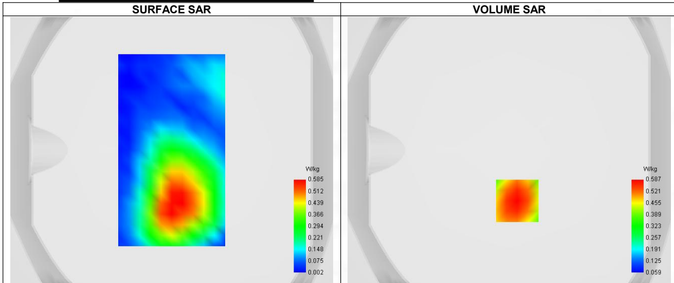
Maximum location: X=6.00, Y=-38.00 ; SAR Peak: 0.81 W/kg
