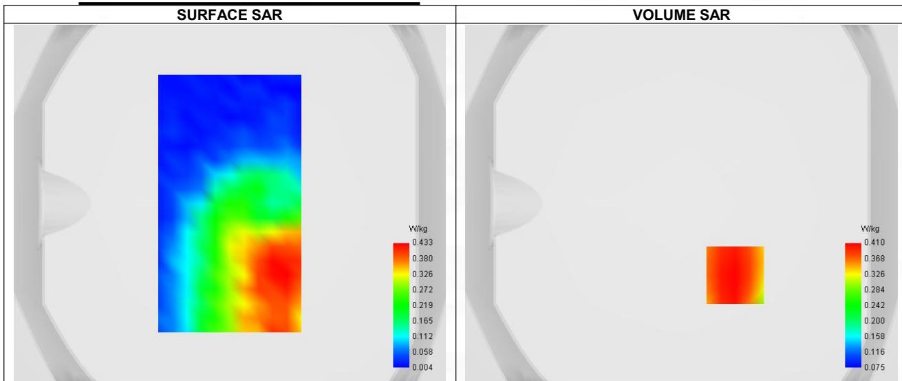
Maximum location: X=30.00, Y=-40.00 ; SAR Peak: 0.50 W/kg
