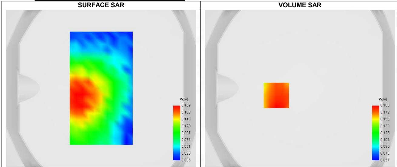
Maximum location: X=-30.00, Y=-9.00 ; SAR Peak: 0.25 W/kg
