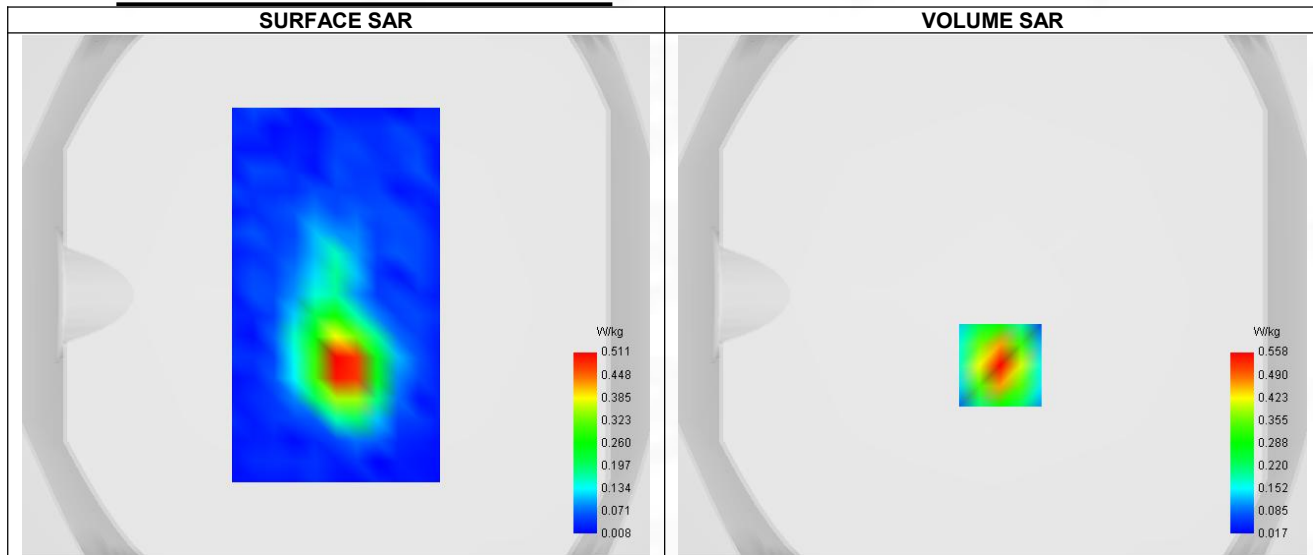
Maximum location: X=3.00, Y=-27.00 ; SAR Peak: 0.91 W/kg
