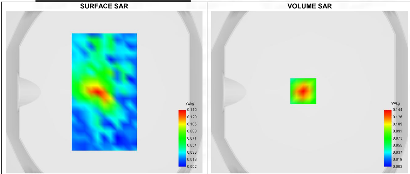
Maximum location: X=-8.00, Y=1.00 ; SAR Peak: 0.27 W/kg
