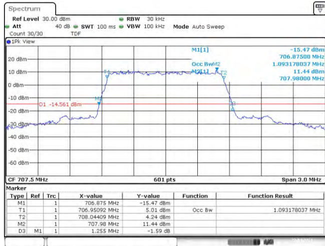
Band12-1.4MHz-QPSK-23095-6RB#0-1.093
