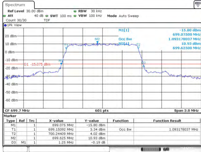
Band12-1.4MHz-QPSK-23017-6RB#0-1.093
