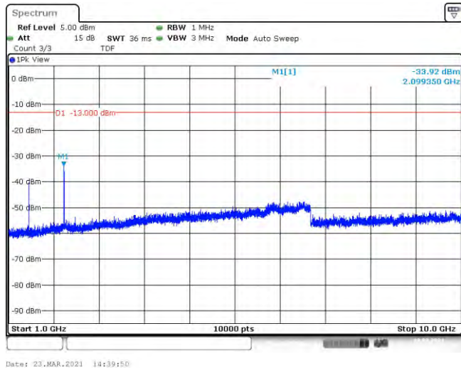
Band12-1.4MHz-QPSK-23095-6RB#0-Range1:30~1000MHz
