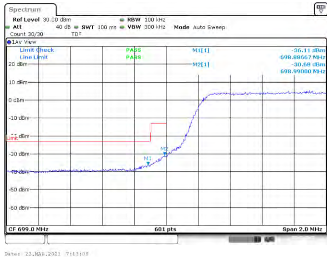
Band12-5MHz-16QAM-23155-25RB#0
