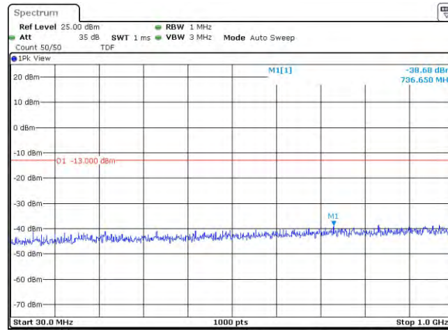
Band2-1.4MHz-QPSK-18607-6RB#0-Range1:30~1000MHz
