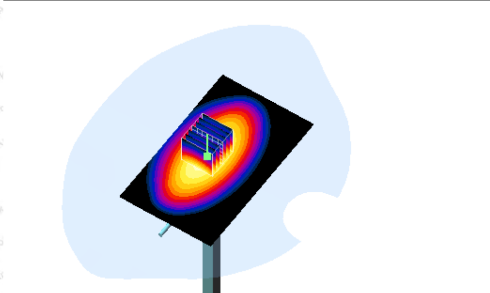
System Performance Check 835MHz Head 250mW
