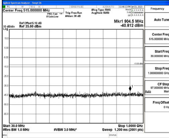
30 MHz – 1000 MHz
