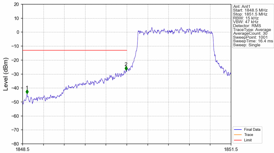
Band2_1.4MHz_QPSK_LCH_1850.7MHz_RB_6_0_NTNV
