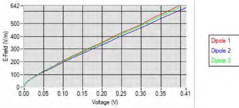
Calibration curves
