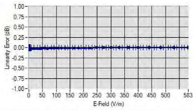
Linearity
