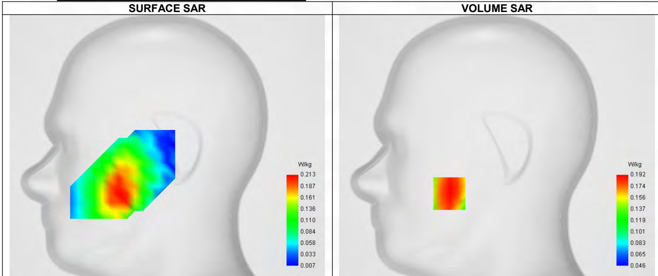
Maximum location: X=-47.00, Y=-47.00 ; SAR Peak: 0.22 W/kg
