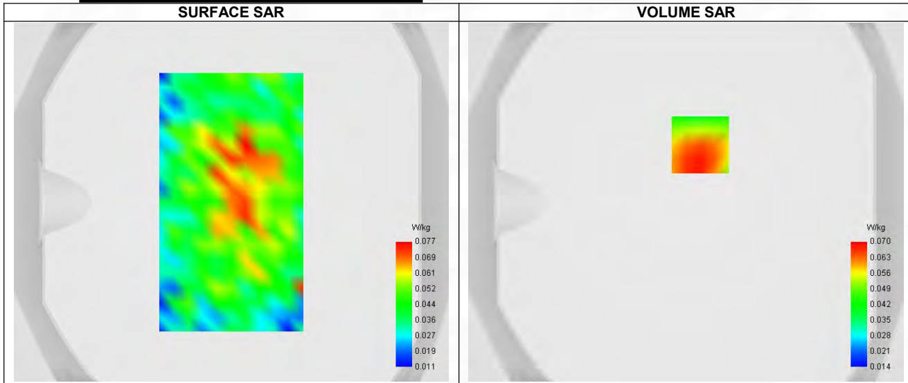
Maximum location: X=8.00, Y=32.00 ; SAR Peak: 0.12 W/kg
