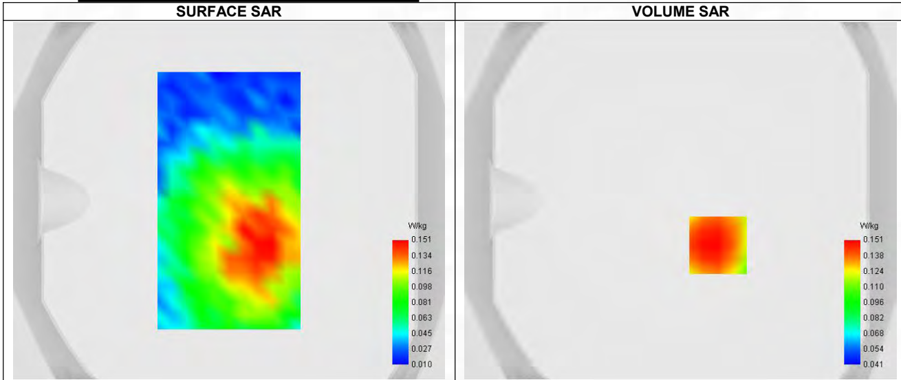
Maximum location: X=21.00, Y=-25.00 ; SAR Peak: 0.20 W/kg
