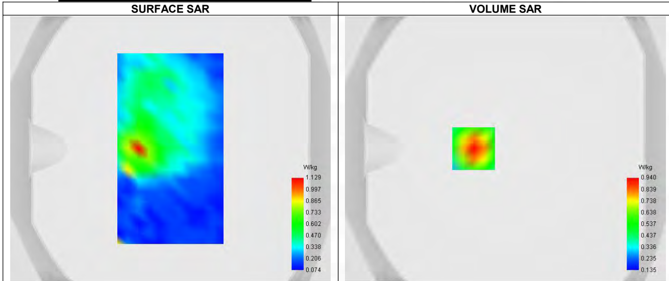
Maximum location: X=-24.00, Y=0.00 ; SAR Peak: 1.45 W/kg
