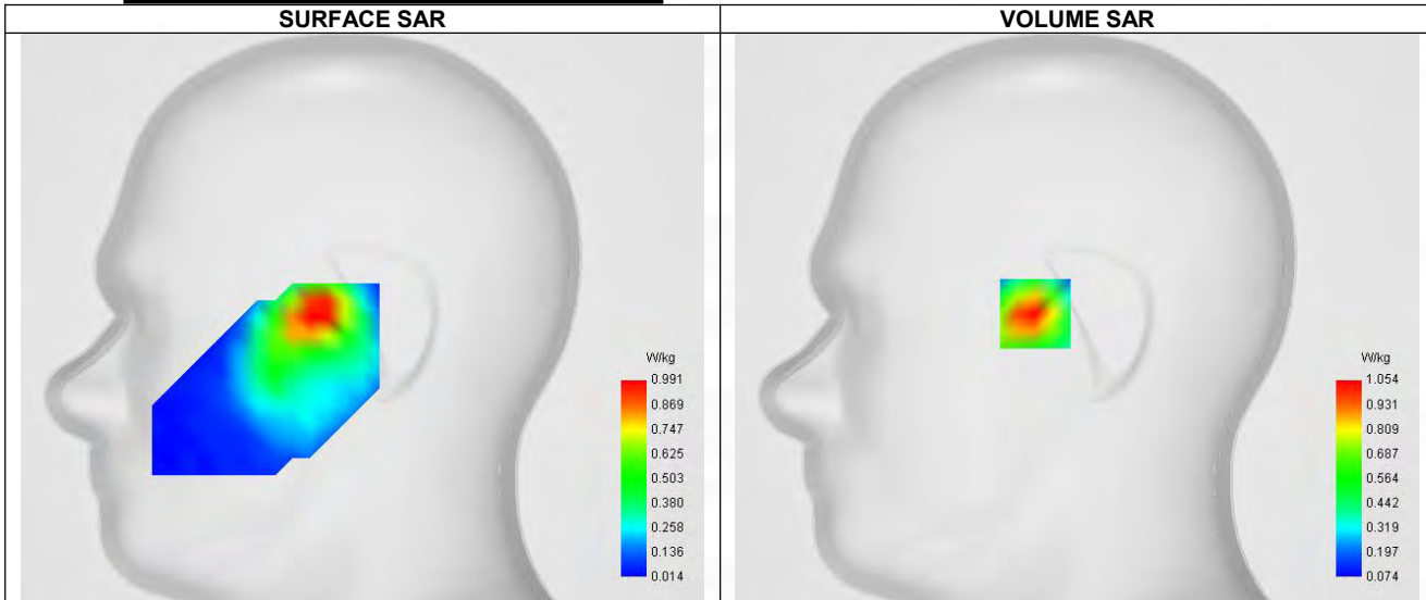
Maximum location: X=-19.00, Y=2.00 ; SAR Peak: 1.53 W/kg
