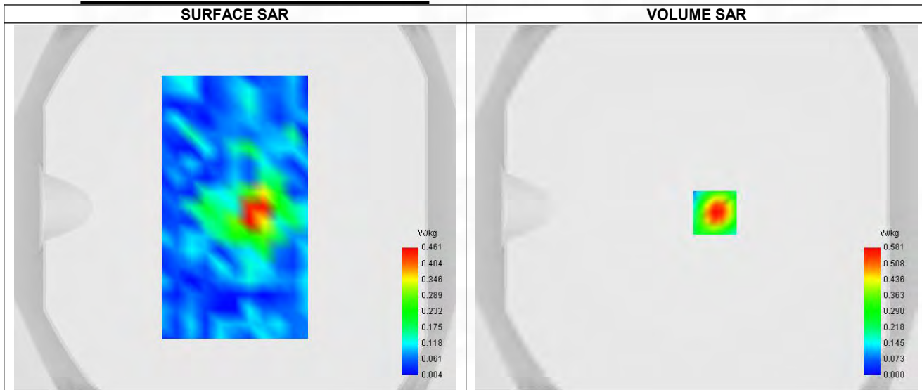
Maximum location: X=10.00, Y=-3.00 ; SAR Peak: 0.92 W/kg
