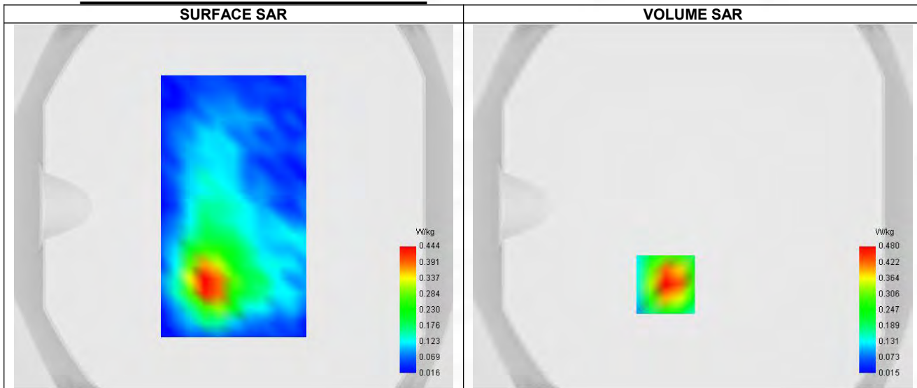
Maximum location: X=-15.00, Y=-43.00 ; SAR Peak: 0.81 W/kg
