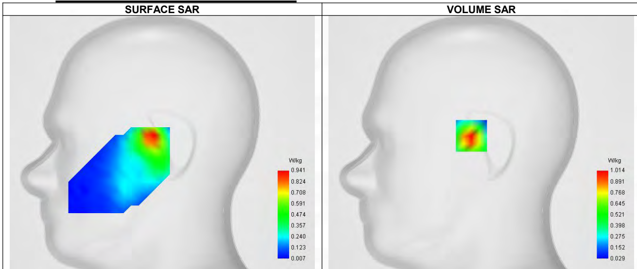
Maximum location: X=-10.00, Y=7.00 ; SAR Peak: 1.58 W/kg
