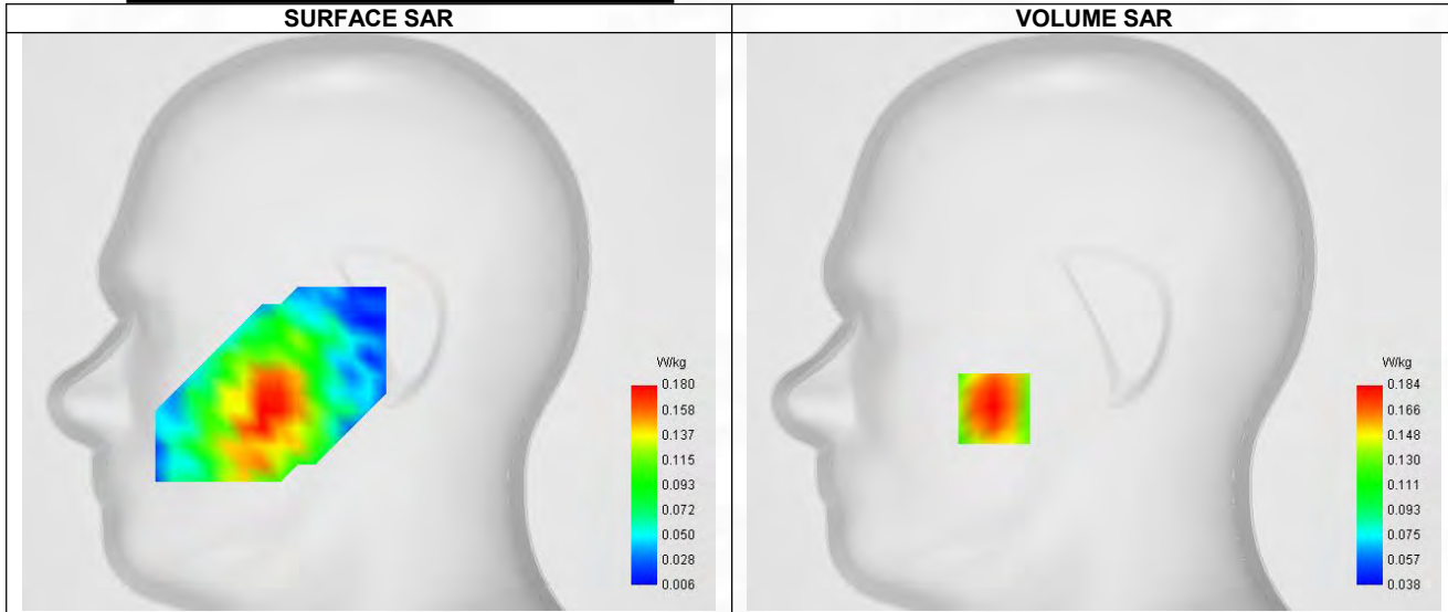
Maximum location: X=-45.00, Y=-39.00 ; SAR Peak: 0.26 W/kg
