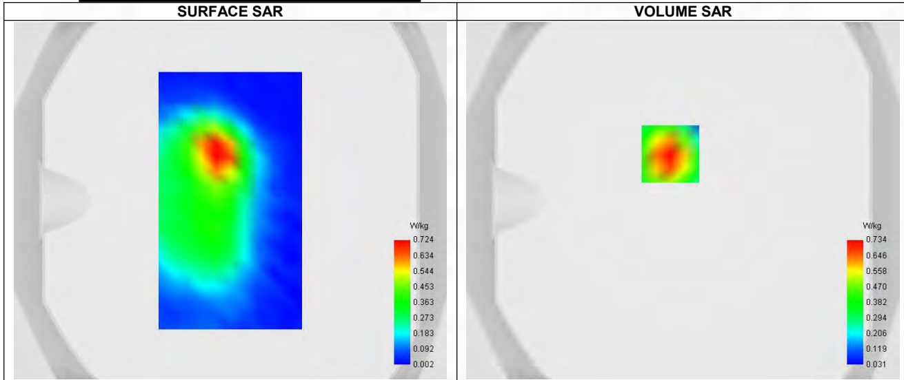
Maximum location: X=-7.00, Y=26.00 ; SAR Peak: 1.10 W/kg
