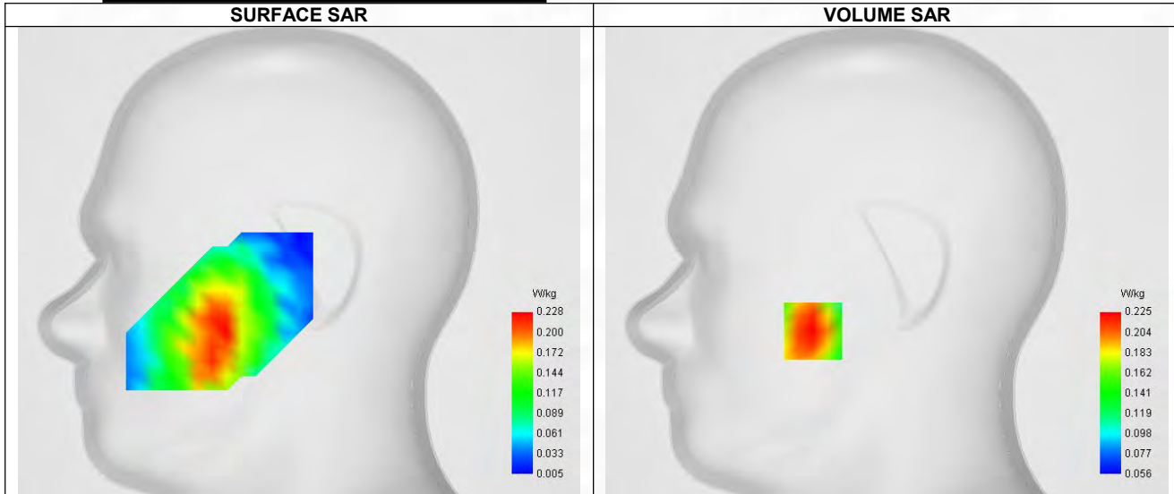
Maximum location: X=-41.00, Y=-39.00 ; SAR Peak: 0.29 W/kg
