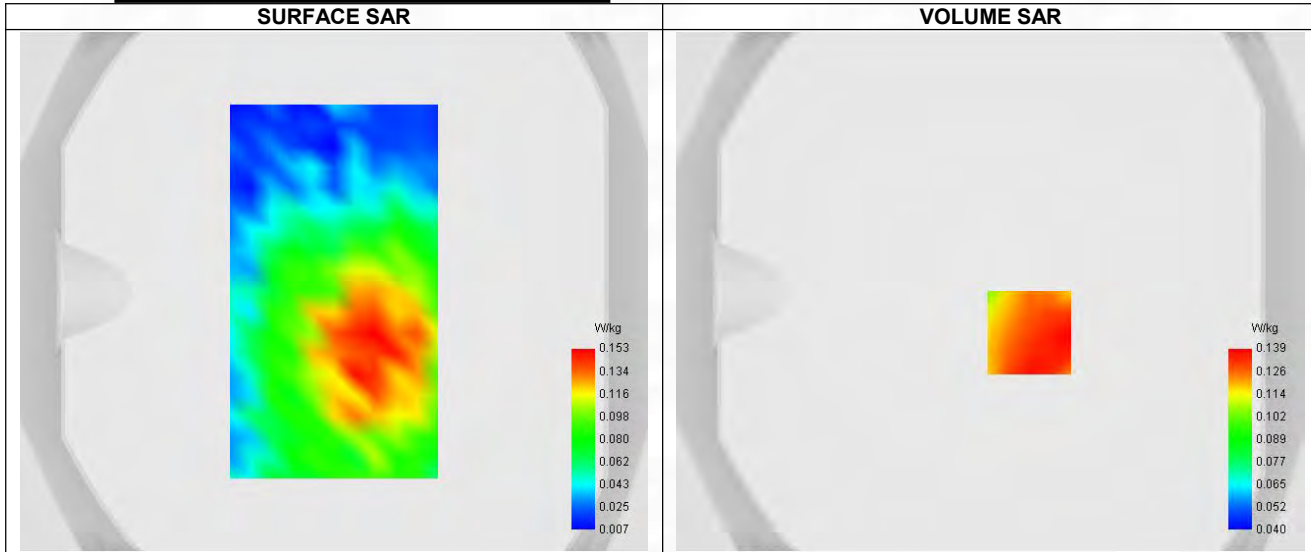
Maximum location: X=15.00, Y=-16.00 ; SAR Peak: 0.20 W/kg
