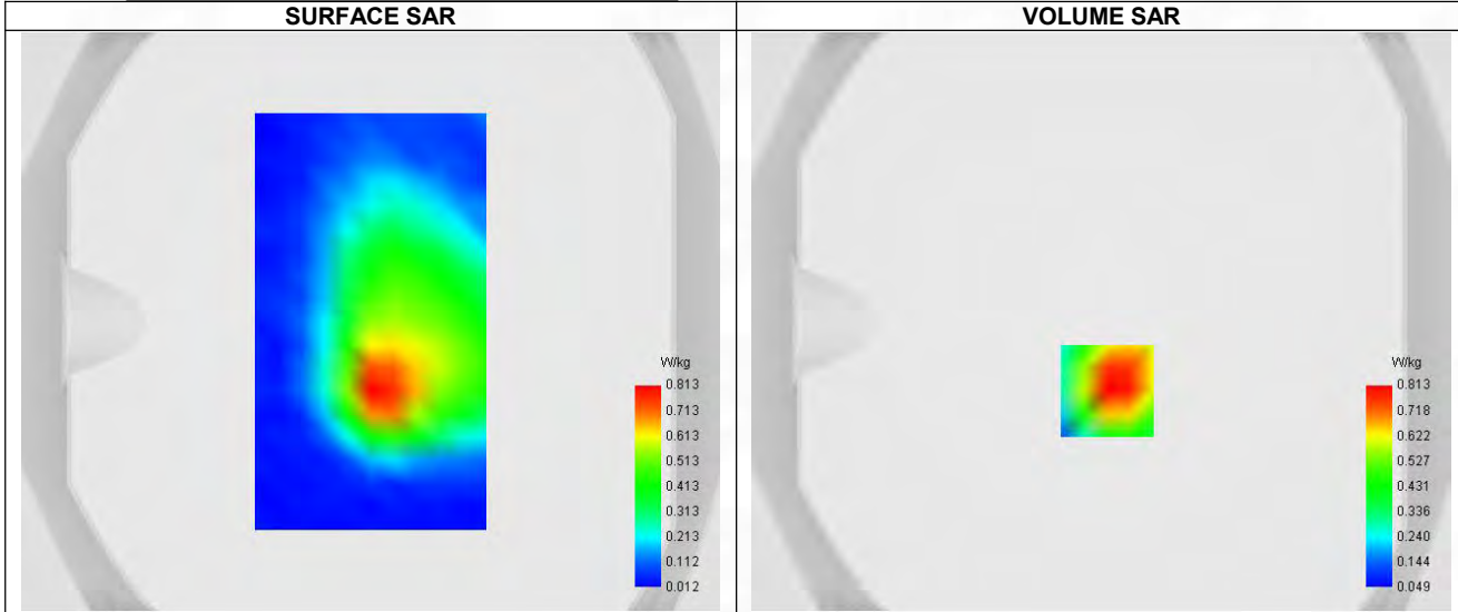
Maximum location: X=2.00, Y=-24.00 ; SAR Peak: 1.27 W/kg
