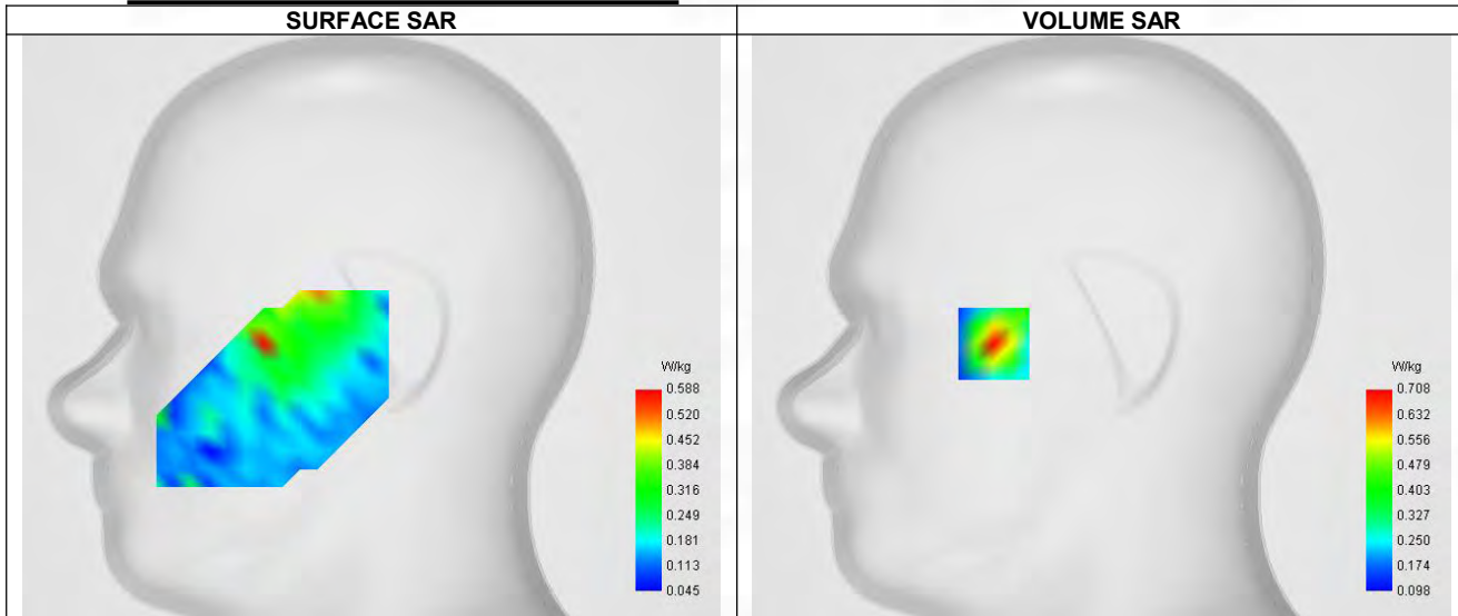
Maximum location: X=-48.00, Y=-8.00 ; SAR Peak: 1.50 W/kg
