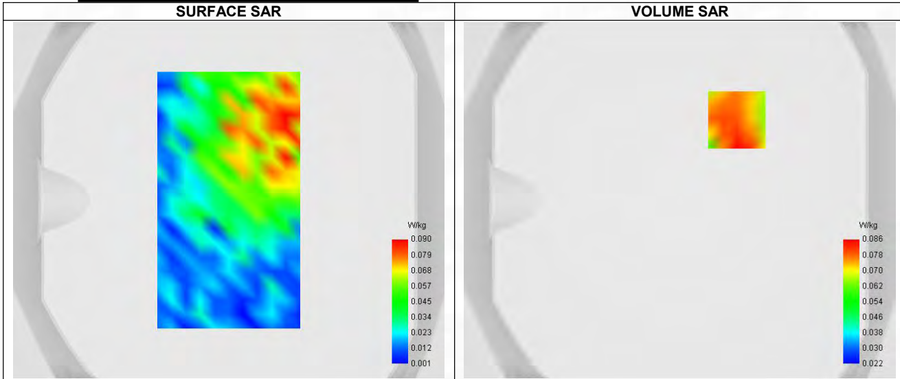
Maximum location: X=32.00, Y=45.00 ; SAR Peak: 0.12 W/kg
