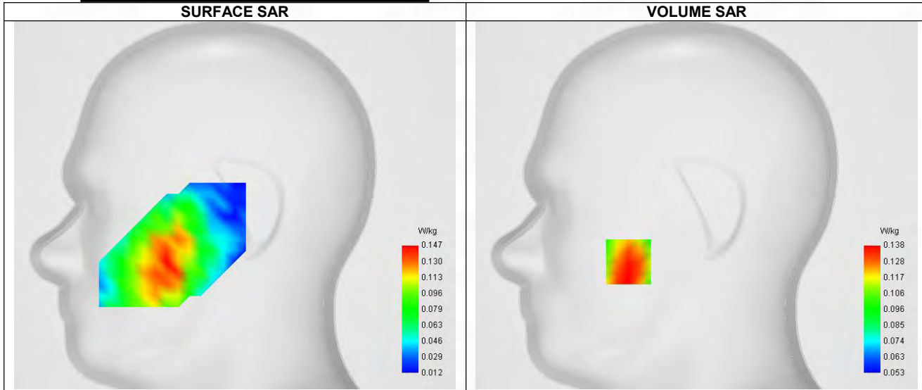
Maximum location: X=-48.00, Y=-40.00 ; SAR Peak: 0.16 W/kg
