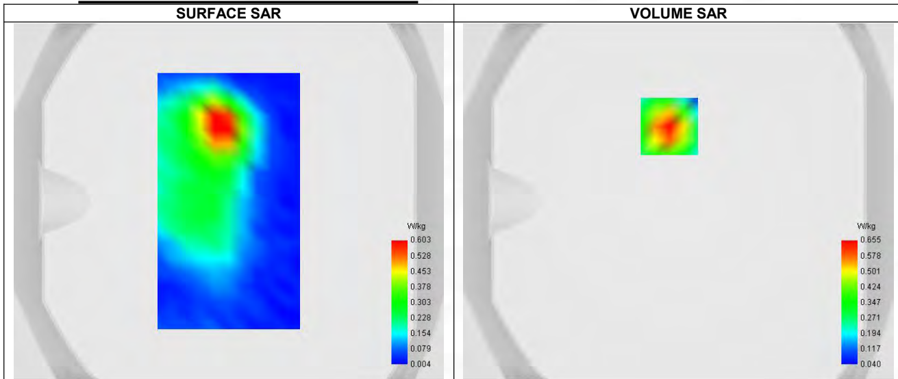
Maximum location: X=-5.00, Y=42.00 ; SAR Peak: 1.05 W/kg
