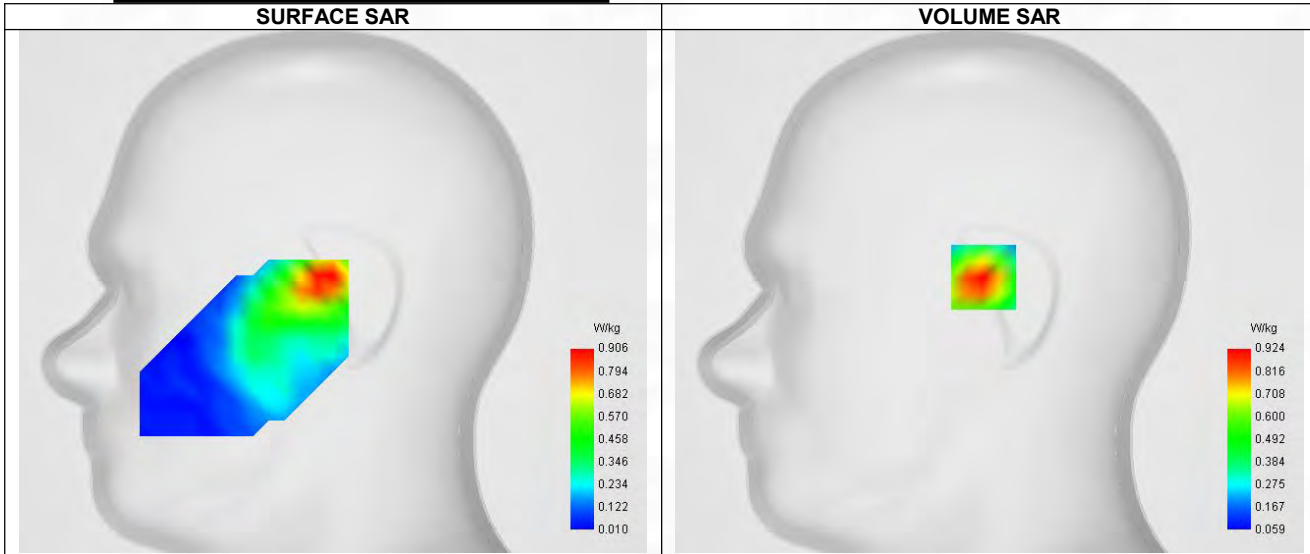
Maximum location: X=-3.00, Y=7.00 ; SAR Peak: 1.30 W/kg
