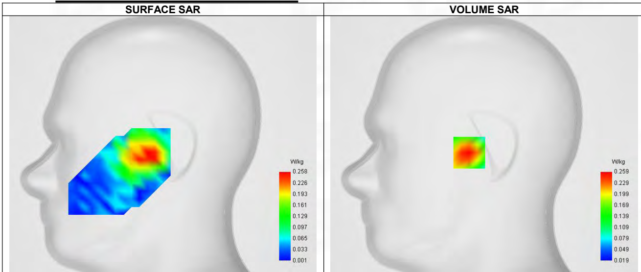
Maximum location: X=-15.00, Y=-9.00 ; SAR Peak: 0.41 W/kg
