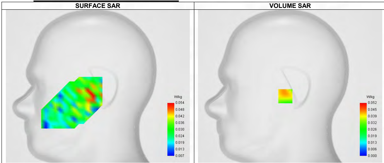
Maximum location: X=-8.00, Y=-17.00 ; SAR Peak: 0.13 W/kg
