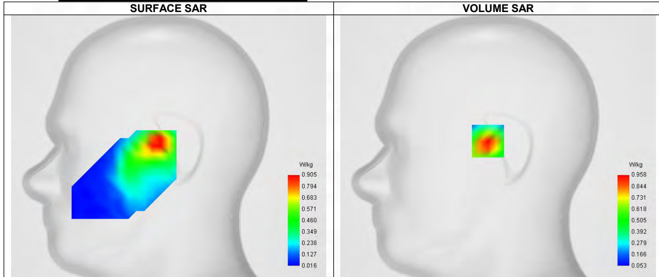
Maximum location: X=-10.00, Y=5.00 ; SAR Peak: 1.42 W/kg
