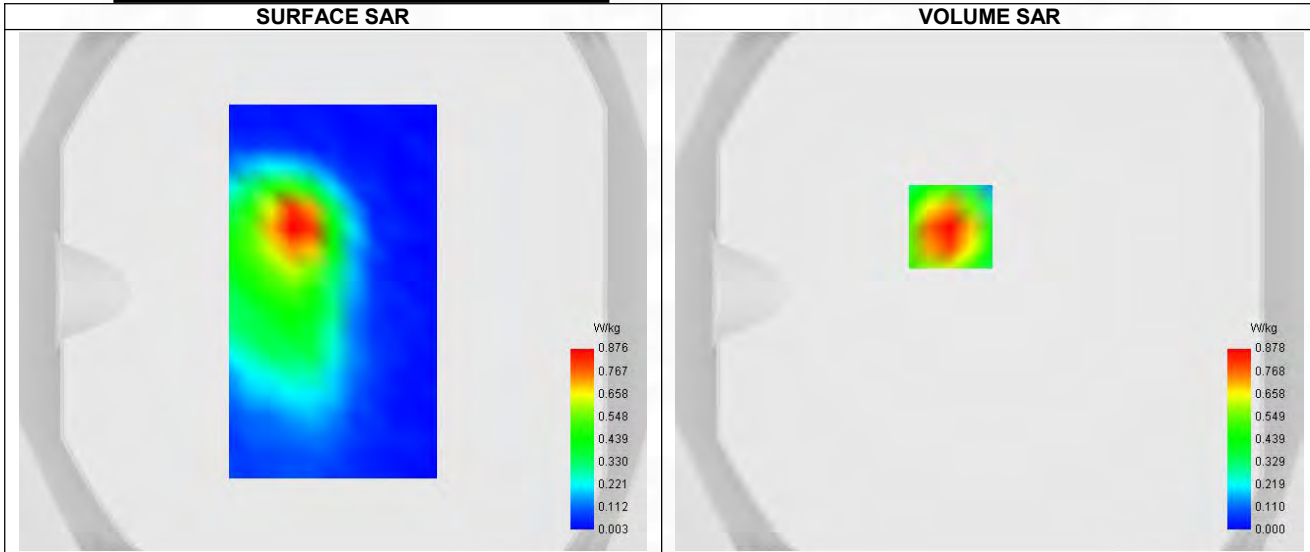
Maximum location: X=-15.00, Y=25.00 ; SAR Peak: 3.40 W/kg
