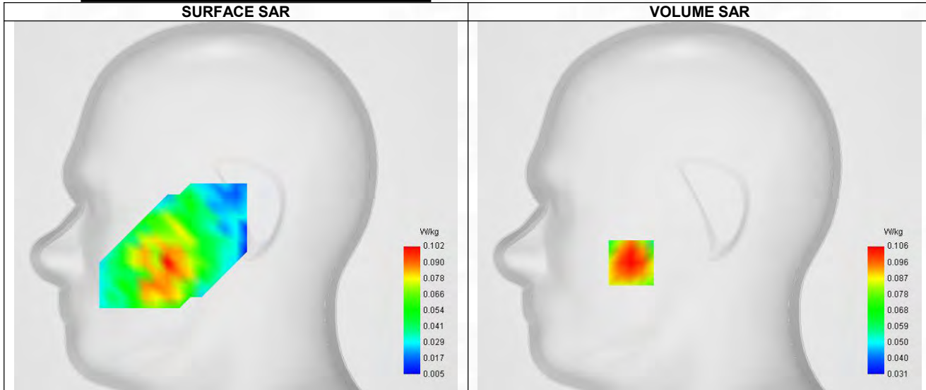
Maximum location: X=-48.00, Y=-40.00 ; SAR Peak: 0.13 W/kg
