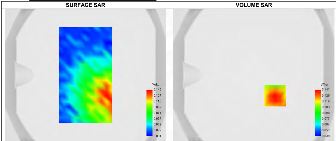
Maximum location: X=32.00, Y=-31.00 ; SAR Peak: 0.19 W/kg
