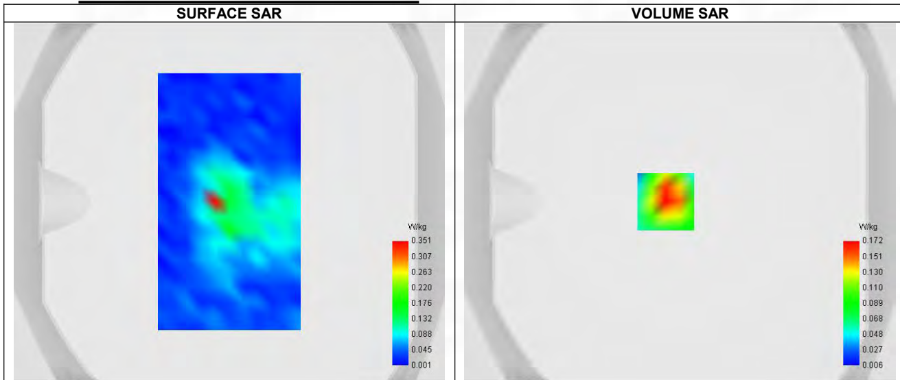
Maximum location: X=-8.00, Y=0.00 ; SAR Peak: 0.33 W/kg
