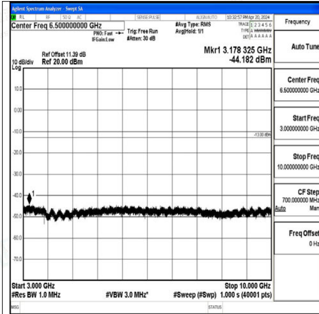
Band71_15MHz_QPSK_133397_1RB#0_3000~10000_3000~10000
