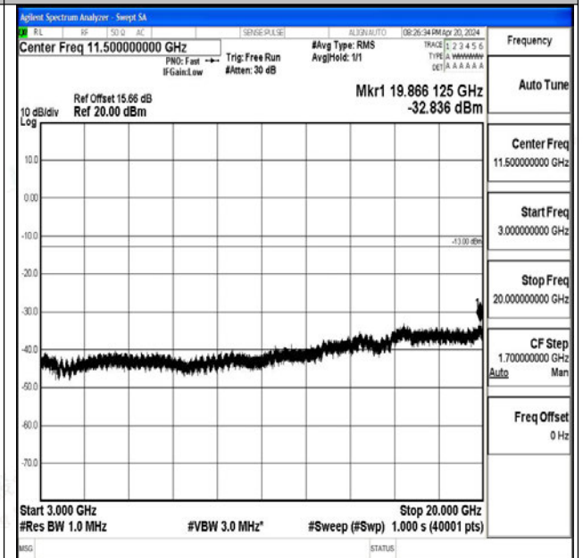
Band66_10MHz_16QAM_132622_1RB#0_3000~20000_3000~20000 3000~20000
