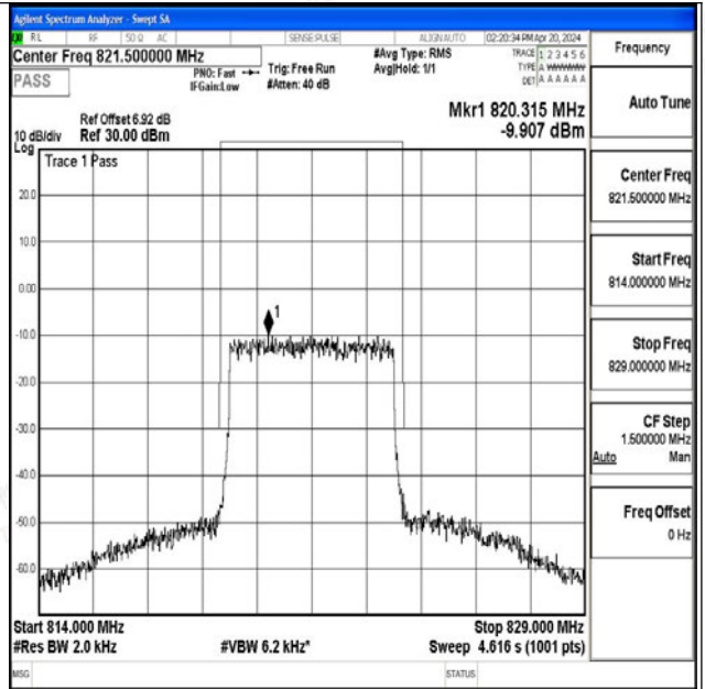
Band26_5MHz_16QAM_26765_25RB#0
